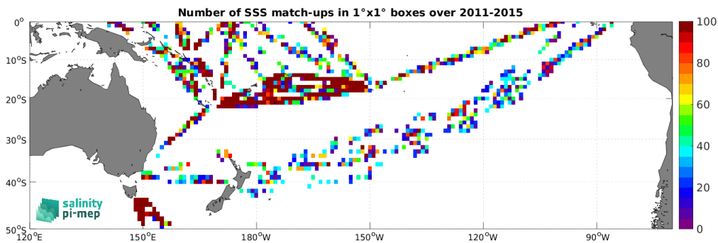
Figure 5: Number of SSS match-ups between TSG (LEGOS-DM) SSS and the Aquarius SSS L2 OR v5 (NASA-GSFC) SSS product for the South Pacific Ocean Pi-MEP region over 1^\circ \times 1^\circ boxes and for the full satellite product period.
