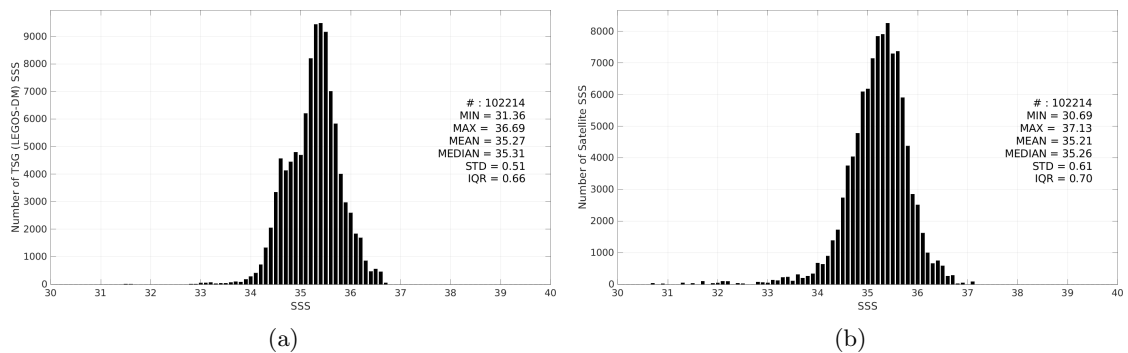
Figure 3: Histograms of SSS from TSG (LEGOS-DM) (a) and Aquarius SSS L2 OR v5 (NASA-GSFC) (b) considering all match-up pairs per bins of 0.1 over the South Pacific Ocean Pi-MEP region and for the full satellite product period.
