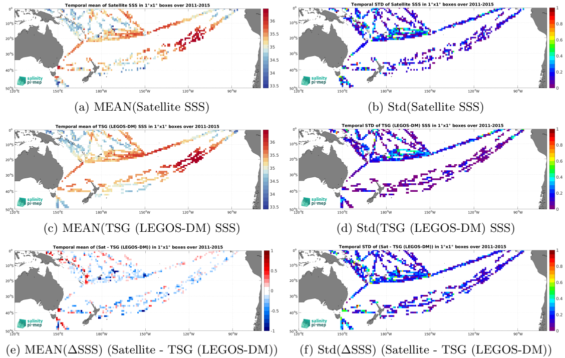
Figure 7: Temporal mean (left) and Std (right) of SSS from Aquarius SSS L2 OR v5 (NASA-GSFC) (top), TSG (LEGOS-DM) (middle), and of \Delta SSS (Satellite - TSG (LEGOS-DM)). Only match-up pairs are used to generate these maps.
