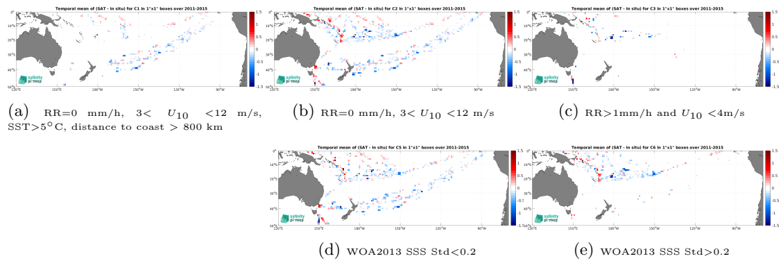
Figure 14: Temporal mean gridded over spatial boxes of size 1^\circ \times 1^\circ of \Delta\text{SSS} (Aquarius SSS L2 OR v5 (NASA-GSFC) - TSG (LEGOS-DM)) for 5 different subdatasets corresponding to:RR=0 mm/h, 3 < U_{10} < 12 m/s, SST>5°C, distance to coast > 800 km (a), RR=0 mm/h, 3 < U_{10} < 12 m/s (b), RR>1mm/h and U_{10} < 4 m/s (c), WOA2013 SSS Std<0.2 (d), WOA2013 SSS Std>0.2 (e).
