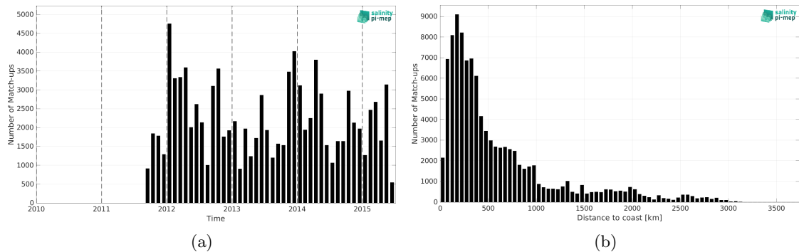
Figure 2: Number of match-ups between TSG (LEGOS-DM) and Aquarius SSS L2 OR v5 (NASA-GSFC) SSS as a function of time (a) and as function of the distance to coast (b) over the South Pacific Ocean Pi-MEP region and for the full satellite product period.
