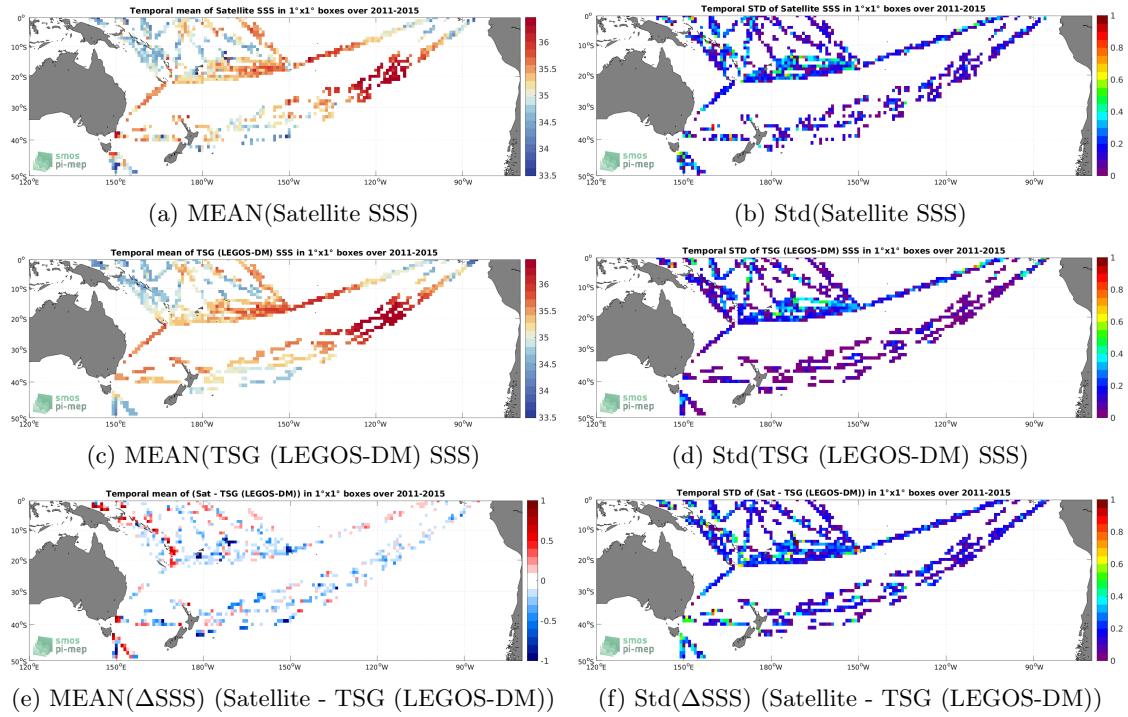
Figure 6: Temporal mean (left) and Std (right) of SSS from Aquarius SSS L2 OR v5 (NASA-GSFC) (top), TSG (LEGOS-DM) (middle), and of \Delta SSS (Satellite - TSG (LEGOS-DM)). Only match-up pairs are used to generate these maps.
