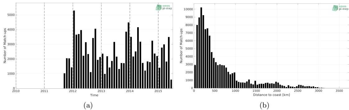
Figure 1: Number of match-ups between TSG (LEGOS-DM) and Aquarius SSS L2 OR v5 (NASA-GSFC) SSS as a function of time (a) and as function of the distance to coast (b) over the South Pacific Ocean Pi-MEP region and for the full satellite product period.
