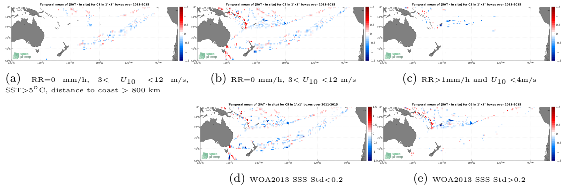
Figure 12: Temporal mean gridded over spatial boxes of size 1^\circ \times 1^\circ of \Delta SSS (Aquarius SSS L2 OR v5 (NASA-GSFC) - TSG (LEGOS-DM)) for 5 different subdatasets corresponding to:RR=0 mm/h, 3 < U_{10} < 12 m/s, SST >5^\circ\text{C} , distance to coast > 800 km (a), RR=0 mm/h, 3 < U_{10} < 12 m/s (b), RR >1 mm/h and U_{10} < 4 m/s (c), WOA2013 SSS Std <0.2 (d), WOA2013 SSS Std >0.2 (e).
