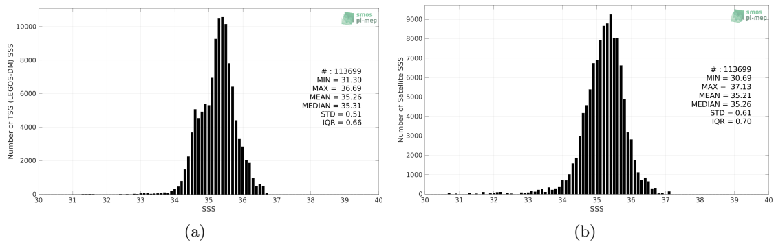
Figure 2: Histograms of SSS from TSG (LEGOS-DM) (a) and Aquarius SSS L2 OR v5 (NASA-GSFC) (b) considering all match-up pairs per bins of 0.1 over the South Pacific Ocean Pi-MEP region and for the full satellite product period.
