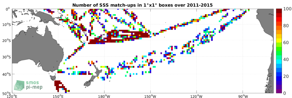
Figure 4: Number of SSS match-ups between TSG (LEGOS-DM) SSS and the Aquarius SSS L2 OR v5 (NASA-GSFC) SSS product for the South Pacific Ocean Pi-MEP region over 1^\circ \times 1^\circ boxes and for the full satellite product period.
