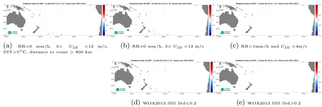
Figure 14: Temporal mean gridded over spatial boxes of size 1^\circ \times 1^\circ of \Delta SSS (Aquarius SSS L2 OR v5 (NASA-GSFC) - TSG (GOSUD-Sailing-ship)) for 5 different subdatasets corresponding to:RR=0 mm/h, 3 < U_{10} < 12 m/s, SST>5°C, distance to coast > 800 km (a), RR=0 mm/h, 3 < U_{10} < 12 m/s (b), RR>1mm/h and U_{10} < 4 m/s (c), WOA2013 SSS Std<0.2 (d), WOA2013 SSS Std>0.2 (e).
