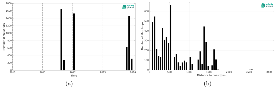
Figure 2: Number of match-ups between TSG (GOSUD-Sailing-ship) and Aquarius SSS L2 OR v5 (NASA-GSFC) SSS as a function of time (a) and as function of the distance to coast (b) over the South Pacific Ocean Pi-MEP region and for the full satellite product period.
