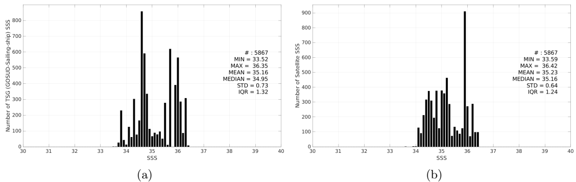
Figure 3: Histograms of SSS from TSG (GOSUD-Sailing-ship) (a) and Aquarius SSS L2 OR v5 (NASA-GSFC) (b) considering all match-up pairs per bins of 0.1 over the South Pacific Ocean Pi-MEP region and for the full satellite product period.
