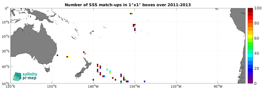
Figure 5: Number of SSS match-ups between TSG (GOSUD-Sailing-ship) SSS and the Aquarius SSS L2 OR v5 (NASA-GSFC) SSS product for the South Pacific Ocean Pi-MEP region over 1^\circ \times 1^\circ boxes and for the full satellite product period.
