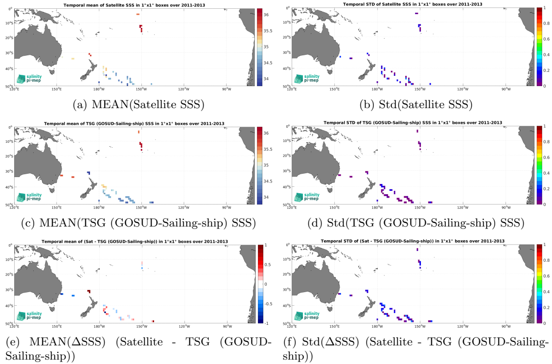
Figure 7: Temporal mean (left) and Std (right) of SSS from Aquarius SSS L2 OR v5 (NASA-GSFC) (top), TSG (GOSUD-Sailing-ship) (middle), and of \Delta SSS (Satellite - TSG (GOSUD-Sailing-ship)). Only match-up pairs are used to generate these maps.
