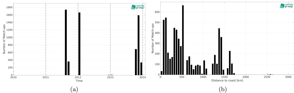
Figure 1: Number of match-ups between TSG (GOSUD-Sailing-ship) and Aquarius SSS L2 OR v5 (NASA-GSFC) SSS as a function of time (a) and as function of the distance to coast (b) over the South Pacific Ocean Pi-MEP region and for the full satellite product period.
