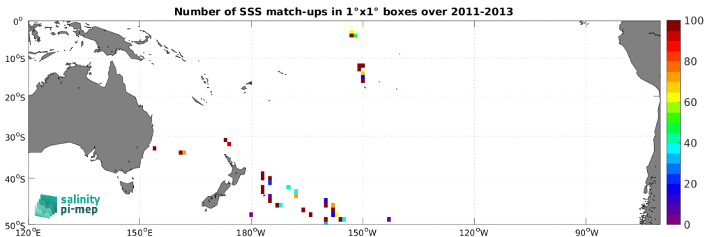
Figure 4: Number of SSS match-ups between TSG (GOSUD-Sailing-ship) SSS and the Aquarius SSS L2 OR v5 (NASA-GSFC) SSS product for the South Pacific Ocean Pi-MEP region over 1^\circ \times 1^\circ boxes and for the full satellite product period.
