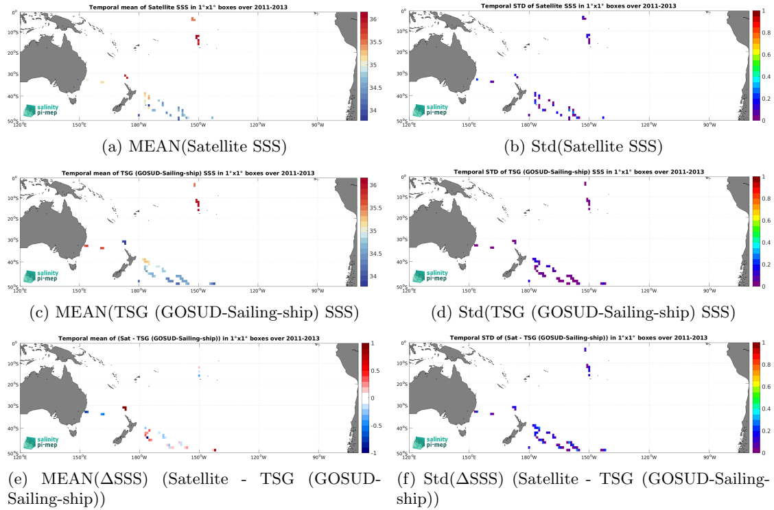
Figure 6: Temporal mean (left) and Std (right) of SSS from Aquarius SSS L2 OR v5 (NASA-GSFC) (top), TSG (GOSUD-Sailing-ship) (middle), and of \Delta SSS (Satellite - TSG (GOSUD-Sailing-ship)). Only match-up pairs are used to generate these maps.
