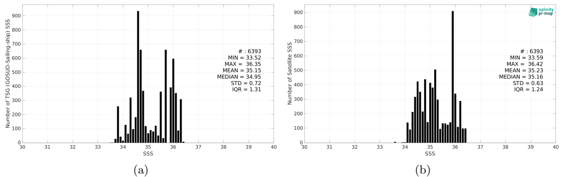
Figure 2: Histograms of SSS from TSG (GOSUD-Sailing-ship) (a) and Aquarius SSS L2 OR v5 (NASA-GSFC) (b) considering all match-up pairs per bins of 0.1 over the South Pacific Ocean Pi-MEP region and for the full satellite product period.
