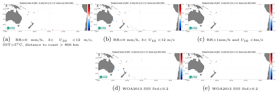
Figure 12: Temporal mean gridded over spatial boxes of size 1^\circ \times 1^\circ of \Delta SSS (Aquarius SSS L2 OR v5 (NASA-GSFC) - TSG (GOSUD-Sailing-ship)) for 5 different subdatasets corresponding to: RR=0 mm/h, 3 < U_{10} < 12 m/s, SST > 5°C, distance to coast > 800 km (a), RR=0 mm/h, 3 < U_{10} < 12 m/s (b), RR > 1mm/h and U_{10} < 4 m/s (c), WOA2013 SSS Std < 0.2 (d), WOA2013 SSS Std > 0.2 (e).
