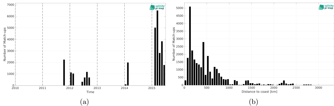
Figure 2: Number of match-ups between TSG (GOSUD-Research-vessel) and Aquarius SSS L2 OR v5 (NASA-GSFC) SSS as a function of time (a) and as function of the distance to coast (b) over the South Pacific Ocean Pi-MEP region and for the full satellite product period.
