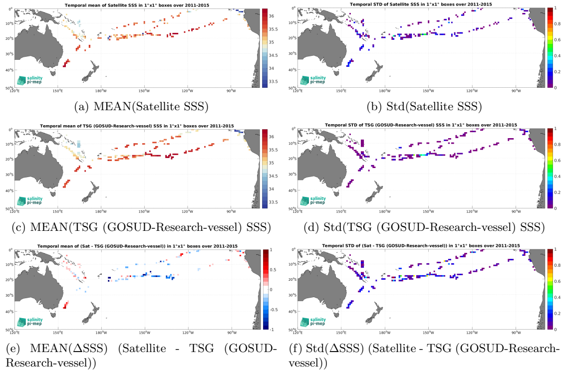
Figure 7: Temporal mean (left) and Std (right) of SSS from Aquarius SSS L2 OR v5 (NASA-GSFC) (top), TSG (GOSUD-Research-vessel) (middle), and of \Delta SSS (Satellite - TSG (GOSUD-Research-vessel)). Only match-up pairs are used to generate these maps.
