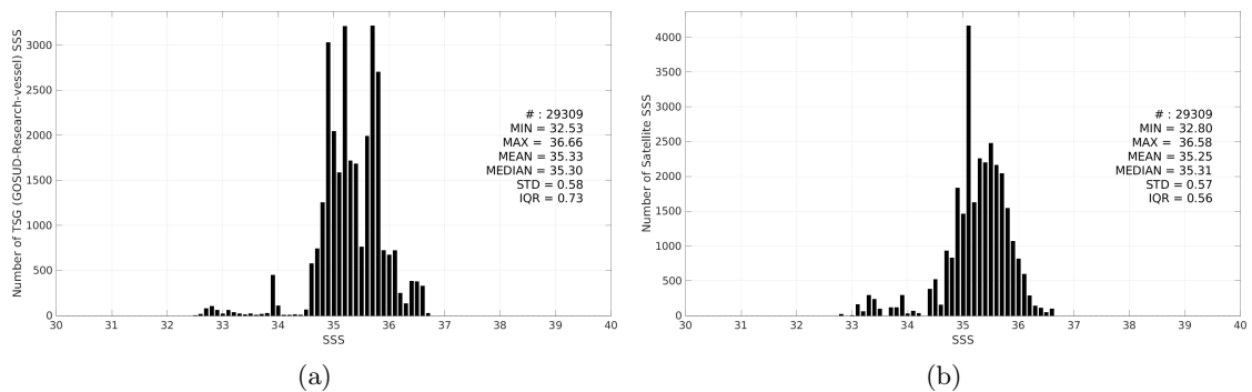
Figure 3: Histograms of SSS from TSG (GOSUD-Research-vessel) (a) and Aquarius SSS L2 OR v5 (NASA-GSFC) (b) considering all match-up pairs per bins of 0.1 over the South Pacific Ocean Pi-MEP region and for the full satellite product period.
