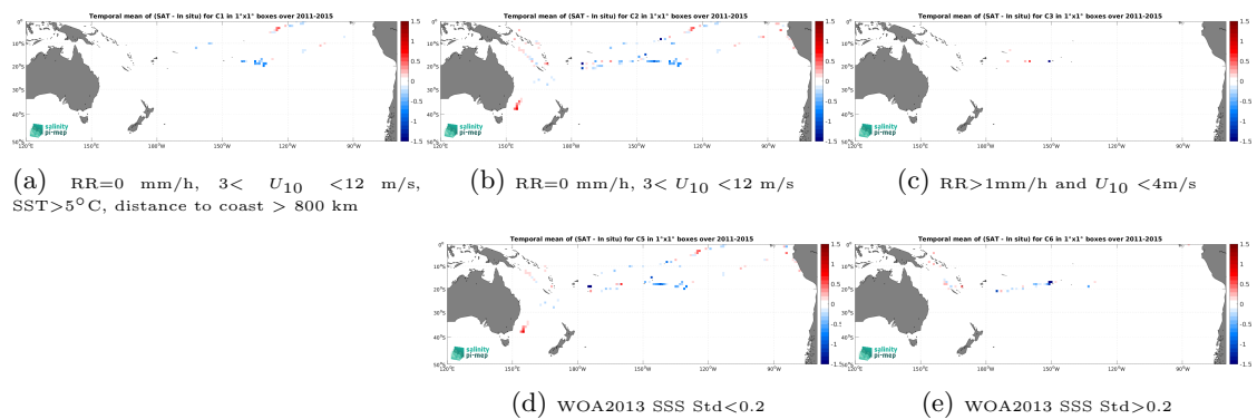
Figure 14: Temporal mean gridded over spatial boxes of size 1^\circ \times 1^\circ of \Delta\text{SSS} (Aquarius SSS L2 OR v5 (NASA-GSFC) - TSG (GOSUD-Research-vessel)) for 5 different subdatasets corresponding to:RR=0 mm/h, 3 < U_{10} < 12 m/s, SST >5^\circ\text{C} , distance to coast > 800 km (a), RR=0 mm/h, 3 < U_{10} < 12 m/s (b), RR >1 mm/h and U_{10} < 4 m/s (c), WOA2013 SSS Std <0.2 (d), WOA2013 SSS Std >0.2 (e).
