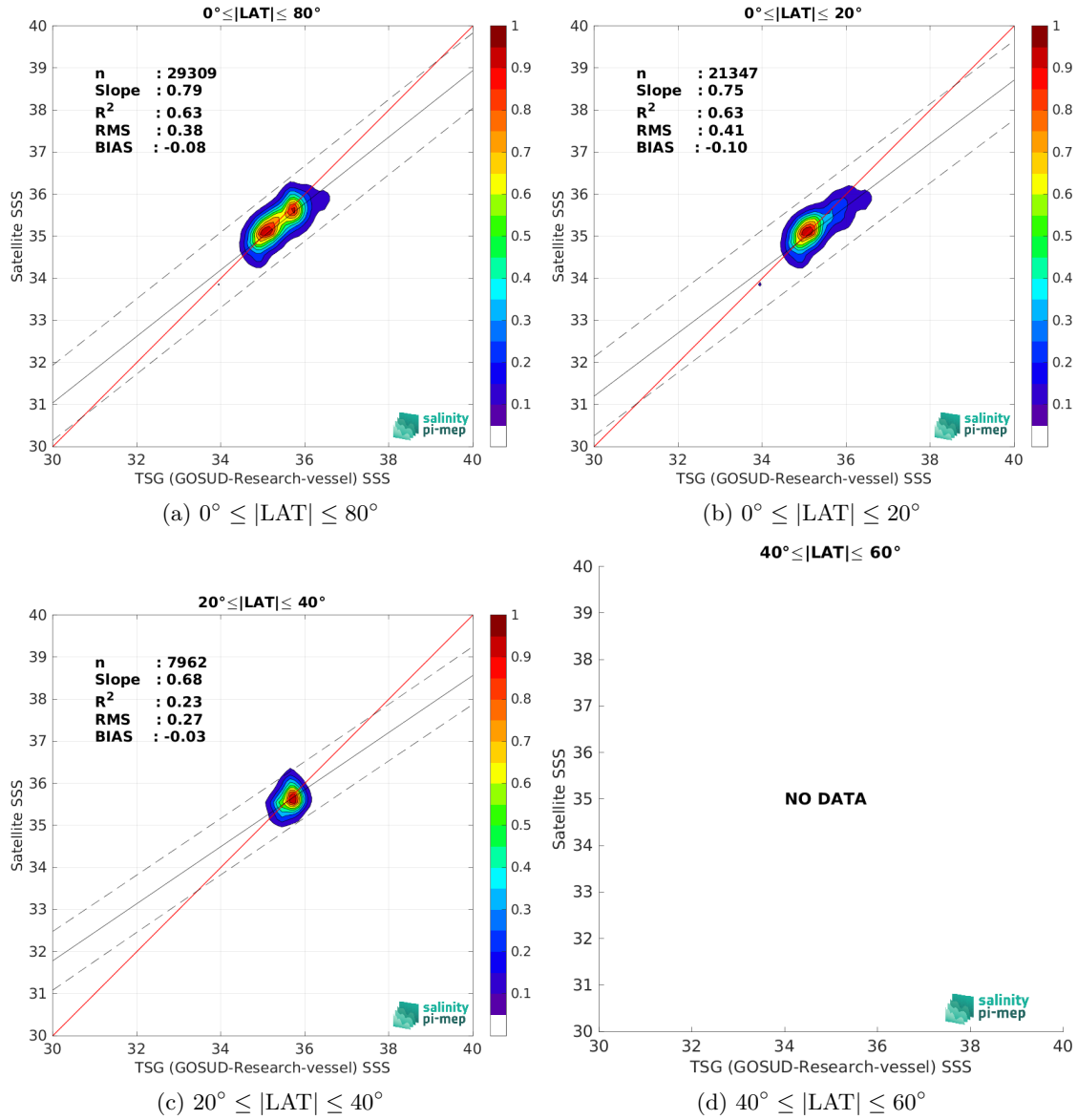
Figure 10: Contour maps of the concentration of Aquarius SSS L2 OR v5 (NASA-GSFC) SSS (y-axis) versus TSG (GOSUD-Research-vessel) SSS (x-axis) at match-up pairs for different latitude bands. For each plot, the red line shows x=y . The black thin and dashed lines indicate a linear fit through the data cloud and the \pm 95\% confidence levels, respectively. The number match-up pairs n , the slope and R^2 coefficient of the linear fit, the root mean square (RMS) and the mean bias between satellite and in situ data are indicated for each latitude band in each plots.
