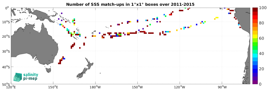
Figure 5: Number of SSS match-ups between TSG (GOSUD-Research-vessel) SSS and the Aquarius SSS L2 OR v5 (NASA-GSFC) SSS product for the South Pacific Ocean Pi-MEP region over 1^\circ \times 1^\circ boxes and for the full satellite product period.
