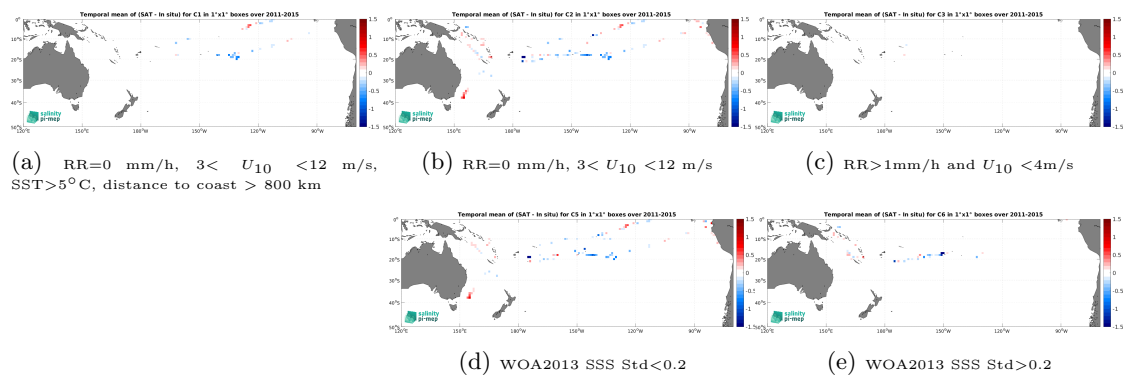
Figure 12: Temporal mean gridded over spatial boxes of size 1^\circ \times 1^\circ of \Delta\text{SSS} (Aquarius SSS L2 OR v5 (NASA-GSFC) - TSG (GOSUD-Research-vessel)) for 5 different subdatasets corresponding to:RR=0 mm/h, 3 < U_{10} < 12 m/s, SST>5°C, distance to coast > 800 km (a), RR=0 mm/h, 3 < U_{10} < 12 m/s (b), RR>1mm/h and U_{10} < 4 m/s (c), WOA2013 SSS Std<0.2 (d), WOA2013 SSS Std>0.2 (e).
