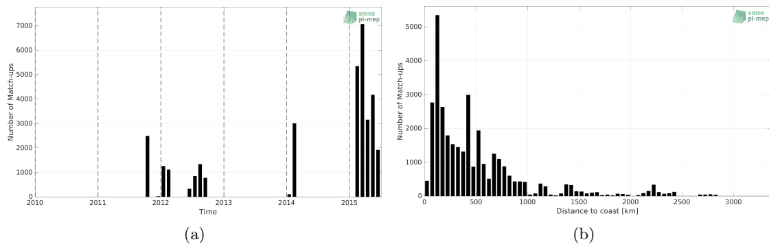
Figure 1: Number of match-ups between TSG (GOSUD-Research-vessel) and Aquarius SSS L2 OR v5 (NASA-GSFC) SSS as a function of time (a) and as function of the distance to coast (b) over the South Pacific Ocean Pi-MEP region and for the full satellite product period.
