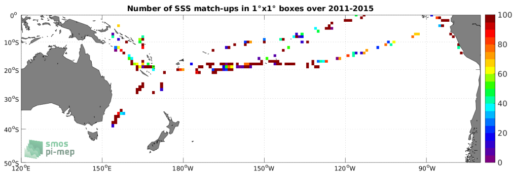
Figure 4: Number of SSS match-ups between TSG (GOSUD-Research-vessel) SSS and the Aquarius SSS L2 OR v5 (NASA-GSFC) SSS product for the South Pacific Ocean Pi-MEP region over 1^\circ \times 1^\circ boxes and for the full satellite product period.
