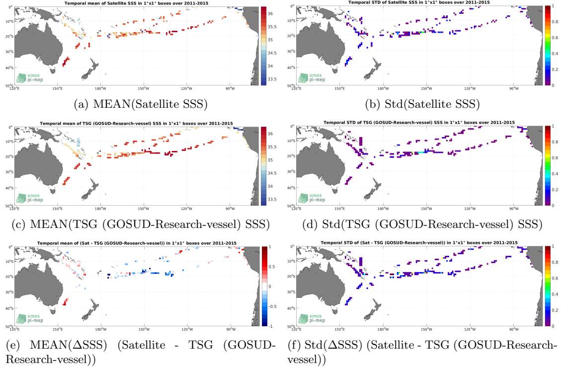
Figure 6: Temporal mean (left) and Std (right) of SSS from Aquarius SSS L2 OR v5 (NASA-GSFC) (top), TSG (GOSUD-Research-vessel) (middle), and of \Delta SSS (Satellite - TSG (GOSUD-Research-vessel)). Only match-up pairs are used to generate these maps.
