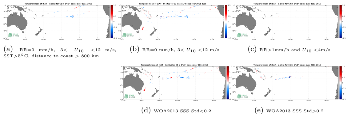
Figure 12: Temporal mean gridded over spatial boxes of size 1^\circ \times 1^\circ of \Delta SSS (Aquarius SSS L2 OR v5 (NASA-GSFC) - TSG (GOSUD-Research-vessel)) for 5 different subdatasets corresponding to: RR=0 mm/h, 3 < U_{10} < 12 m/s, SST >5^\circ\text{C} , distance to coast > 800 km (a), RR=0 mm/h, 3 < U_{10} < 12 m/s (b), RR >1 mm/h and U_{10} < 4 m/s (c), WOA2013 SSS Std <0.2 (d), WOA2013 SSS Std >0.2 (e).
