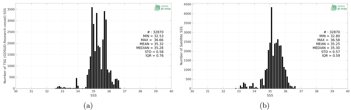
Figure 2: Histograms of SSS from TSG (GOSUD-Research-vessel) (a) and Aquarius SSS L2 OR v5 (NASA-GSFC) (b) considering all match-up pairs per bins of 0.1 over the South Pacific Ocean Pi-MEP region and for the full satellite product period.
