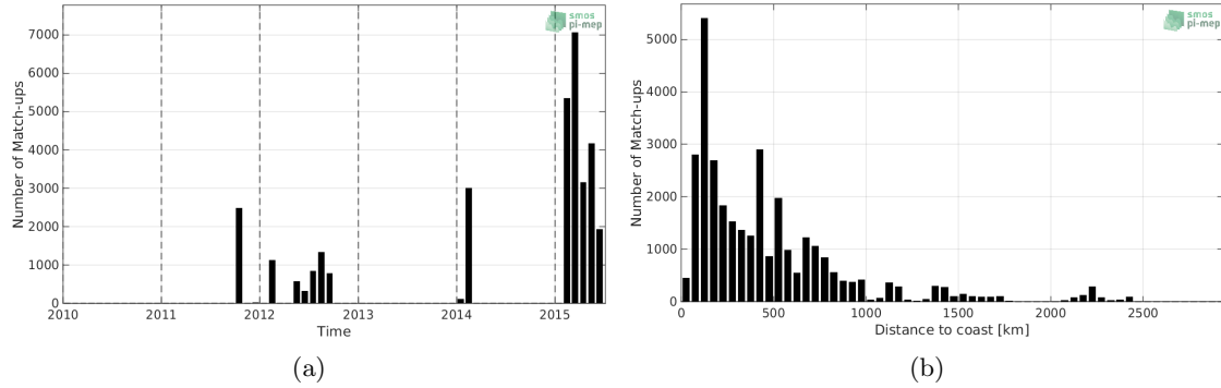
Figure 1: Number of match-ups between TSG-GOSUD-Research-vessel and Aquarius-L2-OR-V5 SSS as a function of time (a) and as function of the distance to coast (b) over the South Pacific Ocean Pi-MEP region and for the full satellite product period.
