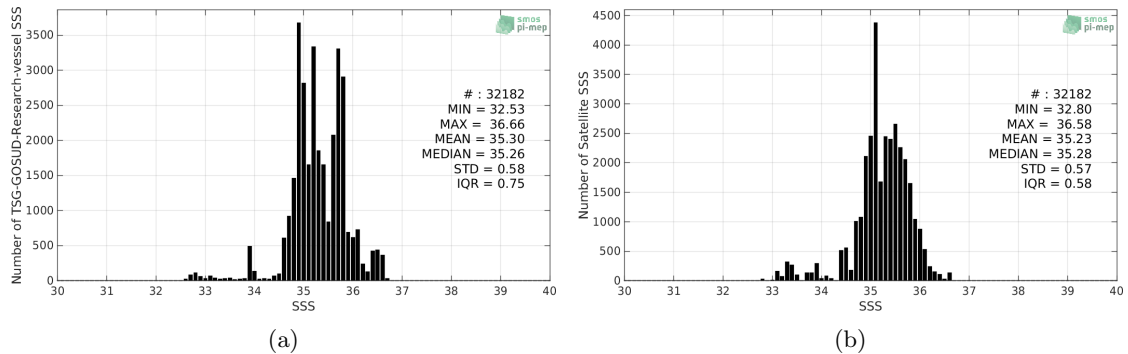
Figure 2: Histograms of SSS from TSG-GOSUD-Research-vessel (a) and Aquarius-L2-OR-V5 (b) considering all match-up pairs per bins of 0.1 over the South Pacific Ocean Pi-MEP region and for the full satellite product period.
