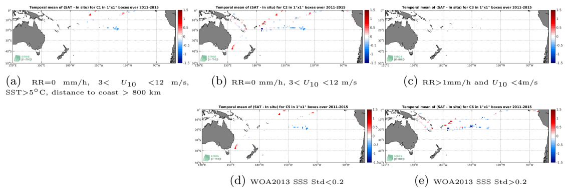
Figure 12: Temporal mean gridded over spatial boxes of size 1^\circ \times 1^\circ of \Delta SSS (Aquarius-L2-OR-V5 - TSG-GOSUD-Research-vessel) for 5 different subdatasets corresponding to:RR=0 mm/h, 3 < U_{10} < 12 m/s, SST >5^\circ\text{C} , distance to coast > 800 km (a), RR=0 mm/h, 3 < U_{10} < 12 m/s (b), RR >1 mm/h and U_{10} < 4 m/s (c), WOA2013 SSS Std <0.2 (d), WOA2013 SSS Std >0.2 (e).
