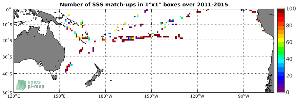
Figure 4: Number of SSS match-ups between TSG-GOSUD-Research-vessel SSS and the Aquarius-L2-OR-V5 SSS product for the South Pacific Ocean Pi-MEP region over 1^\circ \times 1^\circ boxes and for the full satellite product period.
