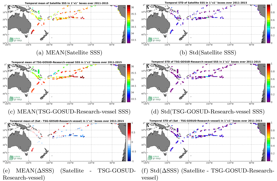
Figure 6: Temporal mean (left) and Std (right) of SSS from Aquarius-L2-OR-V5 (top), TSG-GOSUD-Research-vessel (middle), and of \Delta SSS (Satellite - TSG-GOSUD-Research-vessel). Only match-up pairs are used to generate these maps.
