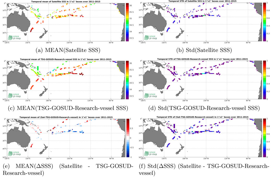
Figure 6: Temporal mean (left) and Std (right) of SSS from Aquarius-L2-OR-V5 (top), TSG-GOSUD-Research-vessel (middle), and of \Delta SSS (Satellite - TSG-GOSUD-Research-vessel). Only match-up pairs are used to generate these maps.
