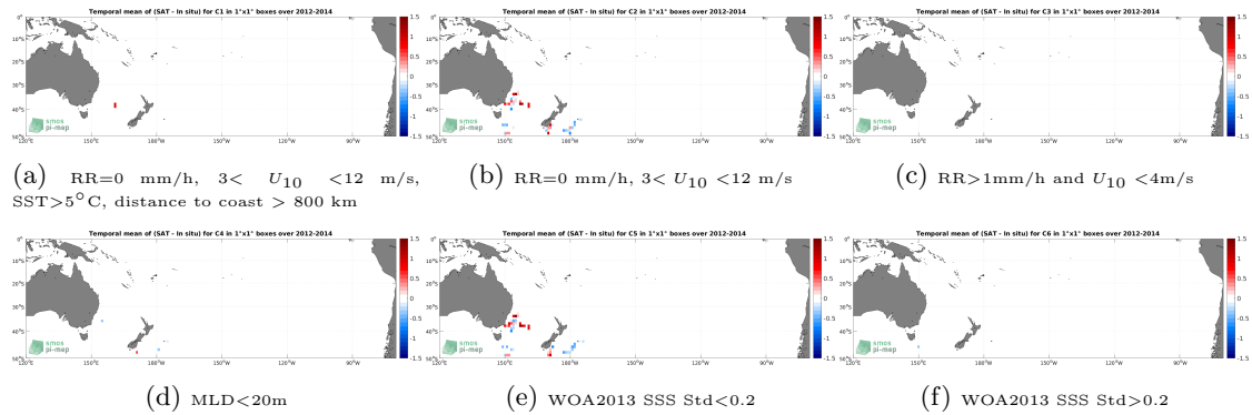
Figure 12: Temporal mean gridded over spatial boxes of size 1^\circ \times 1^\circ of \Delta SSS (Aquarius SSS L2 OR v5 (NASA-GSFC) - Marine mammals) for 6 different subdatasets corresponding to:RR=0 mm/h, 3 < U_{10} < 12 m/s, SST >5^\circ C, distance to coast > 800 km (a), RR=0 mm/h, 3 < U_{10} < 12 m/s (b), RR >1 mm/h and U_{10} < 4 m/s (c),MLD <20 m (d),WOA2013 SSS Std <0.2 (e),WOA2013 SSS Std >0.2 (f).
