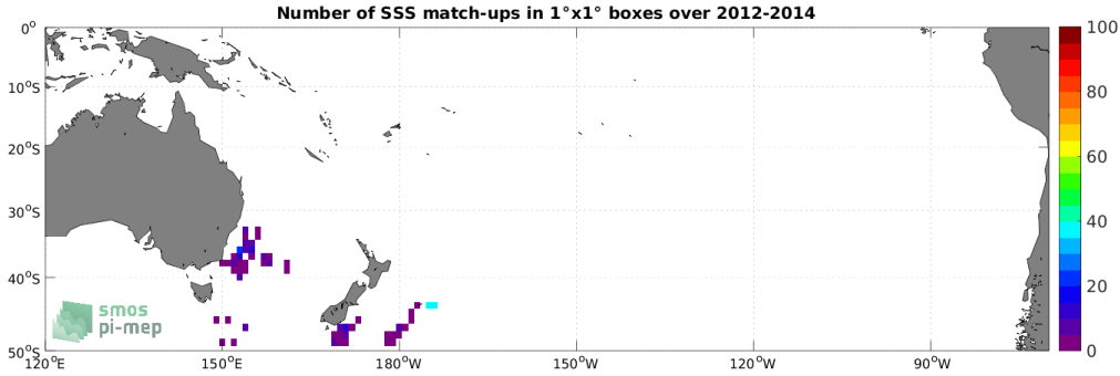
Figure 4: Number of SSS match-ups between Marine mammals SSS and the Aquarius SSS L2 OR v5 (NASA-GSFC) SSS product for the South Pacific Ocean Pi-MEP region over 1^\circ \times 1^\circ boxes and for the full satellite product period.
