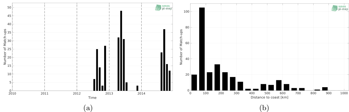
Figure 1: Number of match-ups between Marine mammals and Aquarius SSS L2 OR v5 (NASA-GSFC) SSS as a function of time (a) and as function of the distance to coast (b) over the South Pacific Ocean Pi-MEP region and for the full satellite product period.
