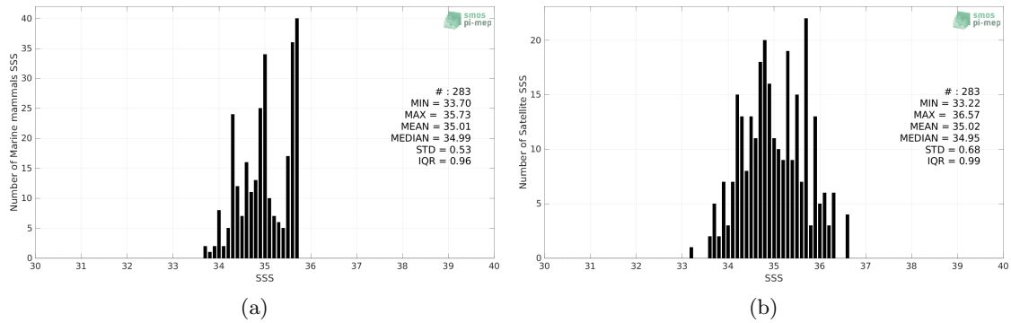
Figure 2: Histograms of SSS from Marine mammals (a) and Aquarius SSS L2 OR v5 (NASA-GSFC) (b) considering all match-up pairs per bins of 0.1 over the South Pacific Ocean Pi-MEP region and for the full satellite product period.
