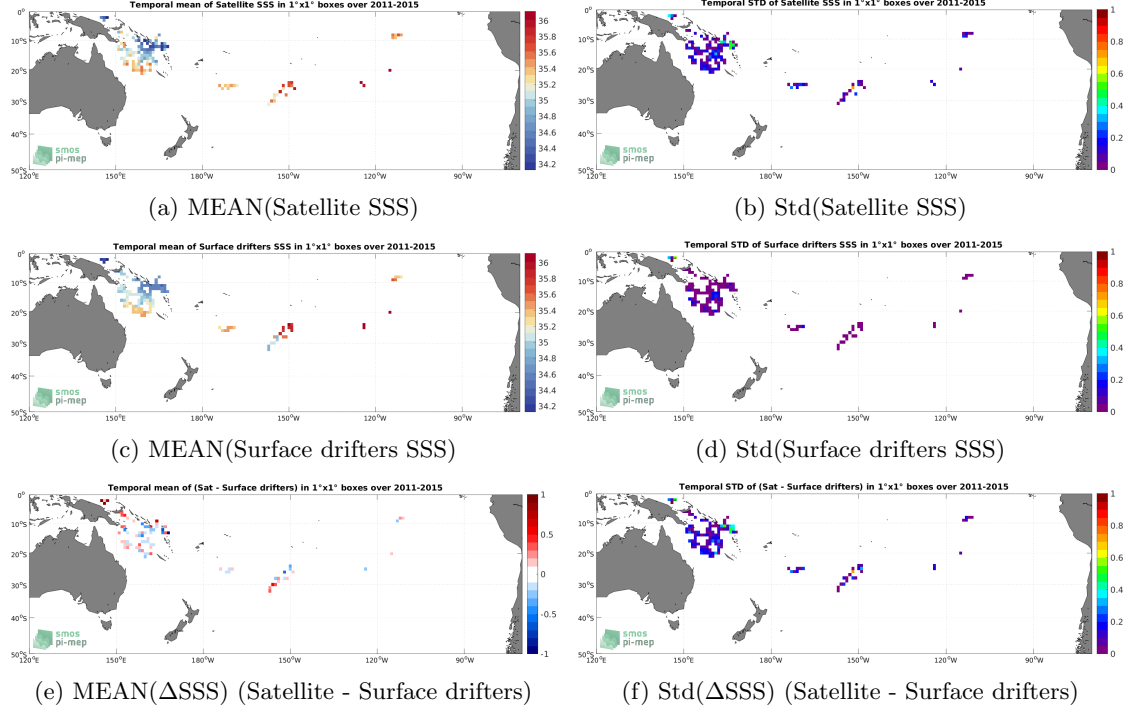
Figure 5: Temporal mean (left) and Std (right) of SSS from Aquarius SSS L2 OR v5 (NASA-GSFC) (top), Surface drifters (middle), and of \Delta\text{SSS} (Satellite - Surface drifters). Only match-up pairs are used to generate these maps.
