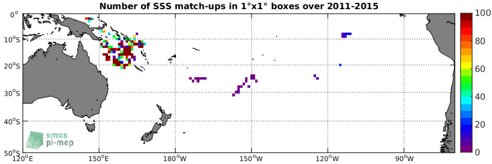
Figure 3: Number of SSS match-ups between Surface drifters SSS and the Aquarius-L2-OR-V5 SSS product for the South Pacific Ocean Pi-MEP region over 1^\circ \times 1^\circ boxes and for the full satellite product period.
