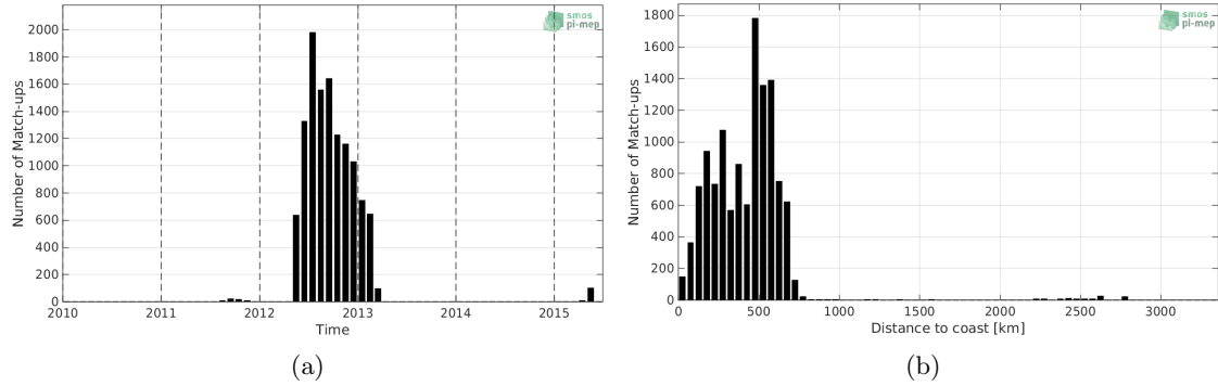
Figure 1: Number of match-ups between Surface drifters and Aquarius-L2-OR-V5 SSS as a function of time (a) and as function of the distance to coast (b) over the South Pacific Ocean Pi-MEP region and for the full satellite product period.
