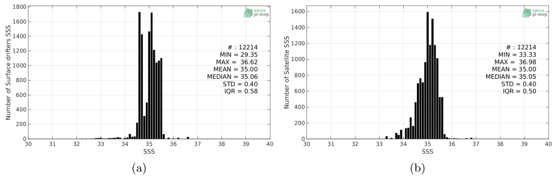
Figure 2: Histograms of SSS from Surface drifters (a) and Aquarius-L2-OR-V5 (b) considering all match-up pairs per bins of 0.1 over the South Pacific Ocean Pi-MEP region and for the full satellite product period.
