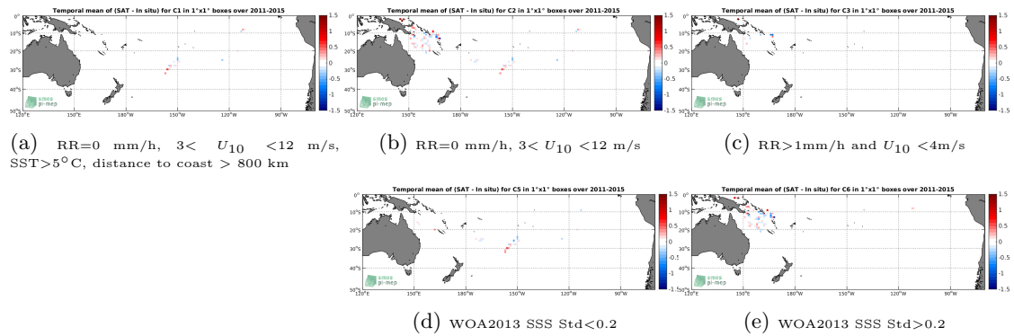
Figure 11: Temporal mean gridded over spatial boxes of size 1^\circ \times 1^\circ of \Delta SSS (Aquarius-L2-OR-V5 - Surface drifters) for 5 different subdatasets corresponding to:RR=0 mm/h, 3 < U_{10} < 12 m/s, SST >5^\circ C, distance to coast > 800 km (a), RR=0 mm/h, 3 < U_{10} < 12 m/s (b), RR >1 mm/h and U_{10} < 4 m/s (c), WOA2013 SSS Std <0.2 (d), WOA2013 SSS Std >0.2 (e).
