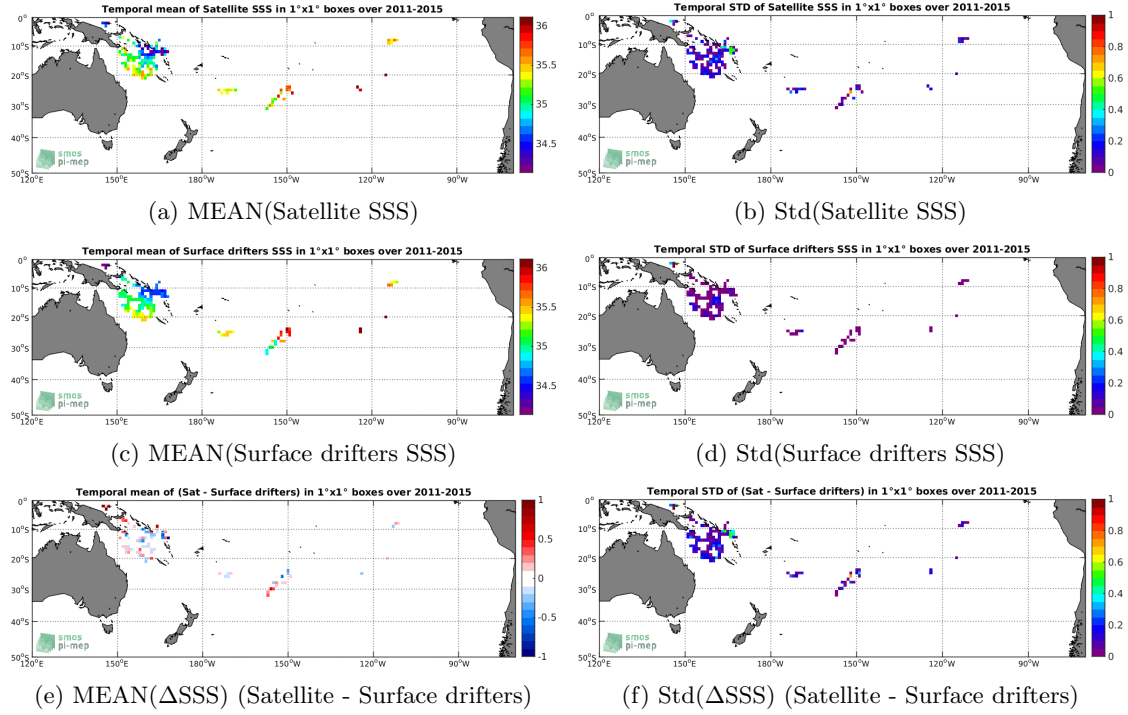
Figure 5: Temporal mean (left) and Std (right) of SSS from Aquarius-L2-OR-V5 (top), Surface drifters (middle), and of \Delta SSS (Satellite - Surface drifters). Only match-up pairs are used to generate these maps.
