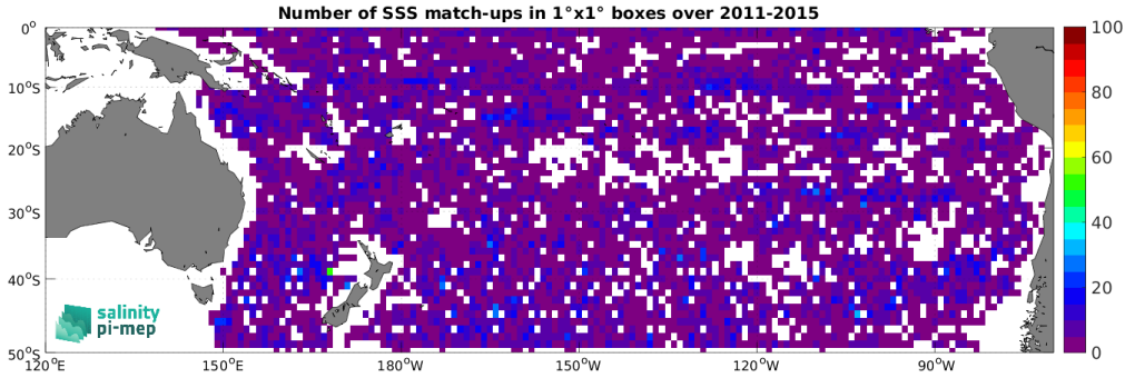
Figure 5: Number of SSS match-ups between Argo SSS and the Aquarius SSS L2 OR v5 (NASA-GSFC) SSS product for the South Pacific Ocean Pi-MEP region over 1^\circ \times 1^\circ boxes and for the full satellite product period.
