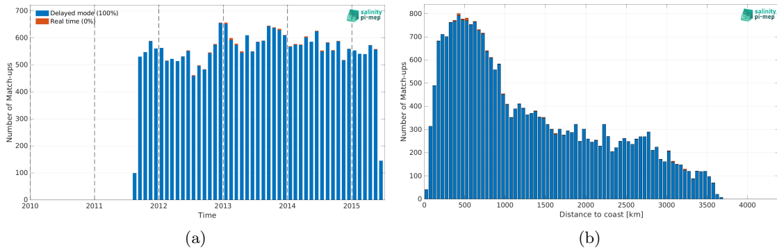
Figure 2: Number of match-ups between Argo and Aquarius SSS L2 OR v5 (NASA-GSFC) SSS as a function of time (a) and as function of the distance to coast (b) over the South Pacific Ocean Pi-MEP region and for the full satellite product period.
