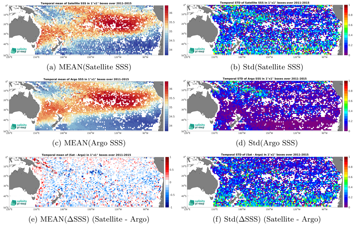
Figure 7: Temporal mean (left) and Std (right) of SSS from Aquarius SSS L2 OR v5 (NASA-GSFC) (top), Argo (middle), and of \Delta SSS (Satellite - Argo). Only match-up pairs are used to generate these maps.
