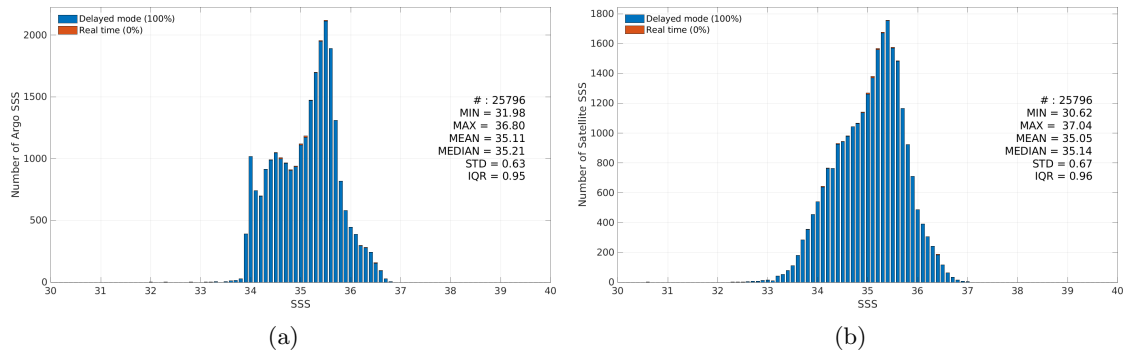
Figure 3: Histograms of SSS from Argo (a) and Aquarius SSS L2 OR v5 (NASA-GSFC) (b) considering all match-up pairs per bins of 0.1 over the South Pacific Ocean Pi-MEP region and for the full satellite product period.
