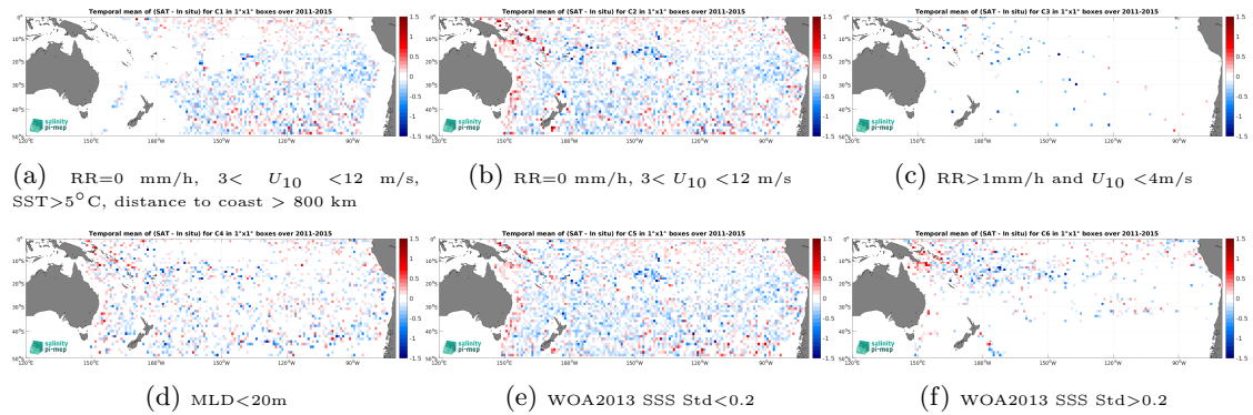
Figure 14: Temporal mean gridded over spatial boxes of size 1^\circ \times 1^\circ of \Delta SSS (Aquarius SSS L2 OR v5 (NASA-GSFC) - Argo) for 6 different subdatasets corresponding to:RR=0 mm/h, 3 < U_{10} < 12 m/s, SST > 5^\circ\text{C} , distance to coast > 800 km (a), RR=0 mm/h, 3 < U_{10} < 12 m/s (b), RR > 1 mm/h and U_{10} < 4 m/s (c),MLD < 20 m (d),WOA2013 SSS Std < 0.2 (e),WOA2013 SSS Std > 0.2 (f).
