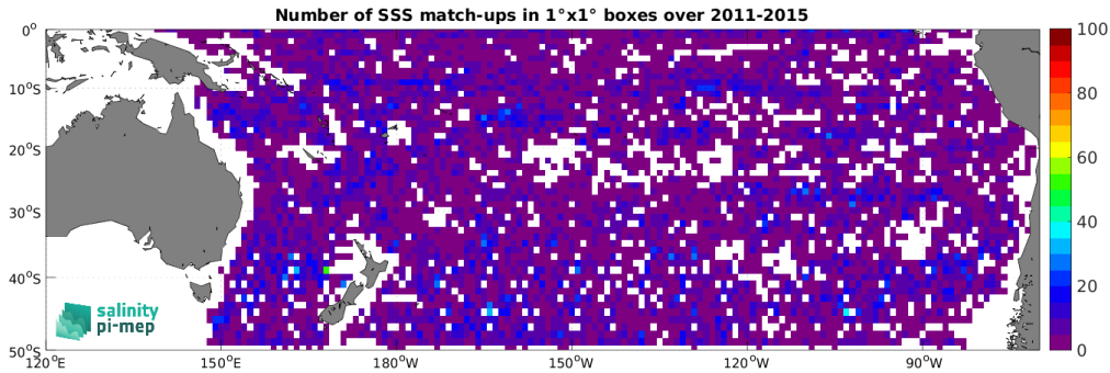
Figure 4: Number of SSS match-ups between Argo SSS and the Aquarius SSS L2 OR v5 (NASA-GSFC) SSS product for the South Pacific Ocean Pi-MEP region over 1^\circ \times 1^\circ boxes and for the full satellite product period.
