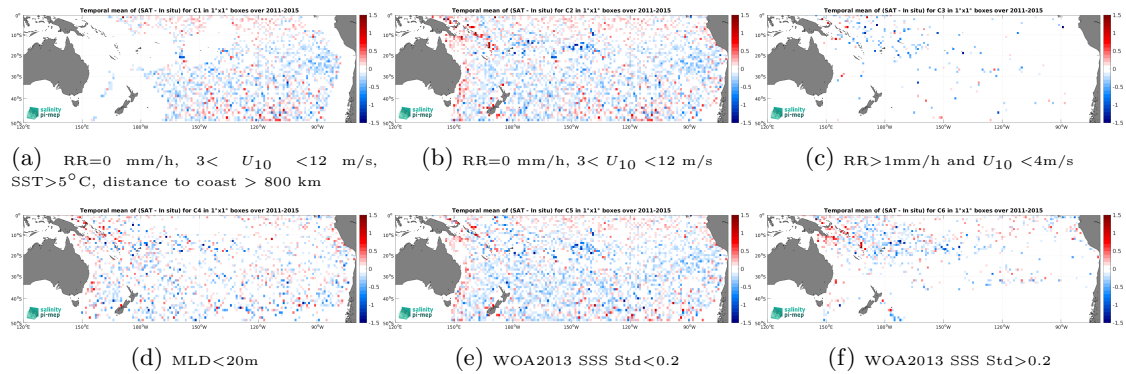
Figure 12: Temporal mean gridded over spatial boxes of size 1^\circ \times 1^\circ of \Delta SSS (Aquarius SSS L2 OR v5 (NASA-GSFC) - Argo) for 6 different subdatasets corresponding to:RR=0 mm/h, 3 < U_{10} < 12 m/s, SST >5^\circ C, distance to coast > 800 km (a), RR=0 mm/h, 3 < U_{10} < 12 m/s (b), RR >1 mm/h and U_{10} < 4 m/s (c),MLD <20 m (d),WOA2013 SSS Std <0.2 (e),WOA2013 SSS Std >0.2 (f).
