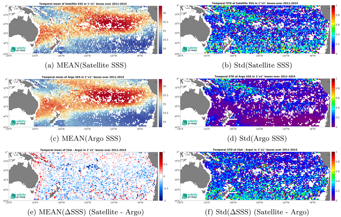
Figure 6: Temporal mean (left) and Std (right) of SSS from Aquarius SSS L2 OR v5 (NASA-GSFC) (top), Argo (middle), and of \Delta SSS (Satellite - Argo). Only match-up pairs are used to generate these maps.
