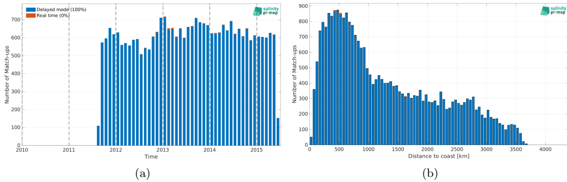
Figure 1: Number of match-ups between Argo and Aquarius SSS L2 OR v5 (NASA-GSFC) SSS as a function of time (a) and as function of the distance to coast (b) over the South Pacific Ocean Pi-MEP region and for the full satellite product period.
