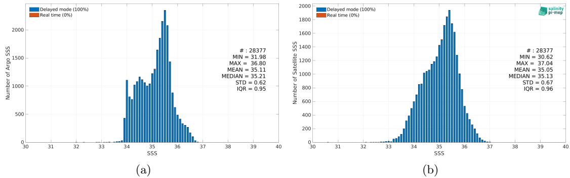
Figure 2: Histograms of SSS from Argo (a) and Aquarius SSS L2 OR v5 (NASA-GSFC) (b) considering all match-up pairs per bins of 0.1 over the South Pacific Ocean Pi-MEP region and for the full satellite product period.
