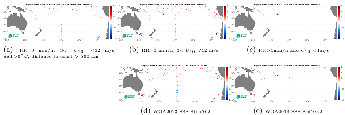
Figure 14: Temporal mean gridded over spatial boxes of size 1^\circ \times 1^\circ of \Delta SSS (Aquarius SSS L2 CAP v5 (JPL) - TSG (SAMOS)) for 5 different subdatasets corresponding to:RR=0 mm/h, 3 < U_{10} < 12 m/s, SST >5^\circ\text{C} , distance to coast > 800 km (a), RR=0 mm/h, 3 < U_{10} < 12 m/s (b), RR >1 mm/h and U_{10} < 4 m/s (c), WOA2013 SSS Std <0.2 (d), WOA2013 SSS Std >0.2 (e).
