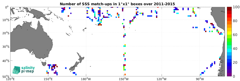
Figure 5: Number of SSS match-ups between TSG (SAMOS) SSS and the Aquarius SSS L2 CAP v5 (JPL) SSS product for the South Pacific Ocean Pi-MEP region over 1^\circ \times 1^\circ boxes and for the full satellite product period.
