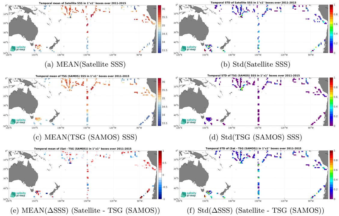
Figure 7: Temporal mean (left) and Std (right) of SSS from Aquarius SSS L2 CAP v5 (JPL) (top), TSG (SAMOS) (middle), and of \Delta SSS (Satellite - TSG (SAMOS)). Only match-up pairs are used to generate these maps.
