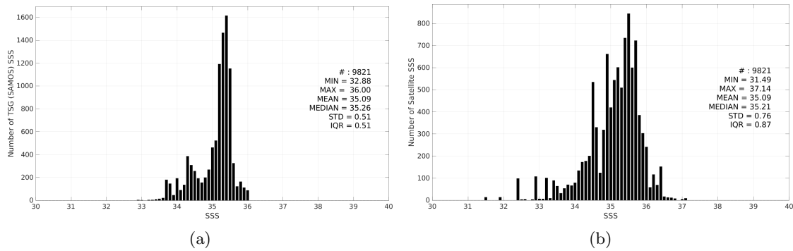
Figure 3: Histograms of SSS from TSG (SAMOS) (a) and Aquarius SSS L2 CAP v5 (JPL) (b) considering all match-up pairs per bins of 0.1 over the South Pacific Ocean Pi-MEP region and for the full satellite product period.
