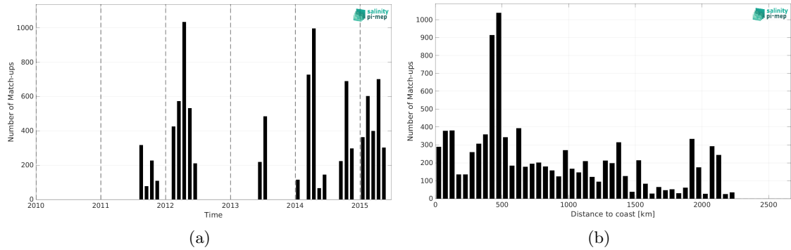
Figure 2: Number of match-ups between TSG (SAMOS) and Aquarius SSS L2 CAP v5 (JPL) SSS as a function of time (a) and as function of the distance to coast (b) over the South Pacific Ocean Pi-MEP region and for the full satellite product period.
