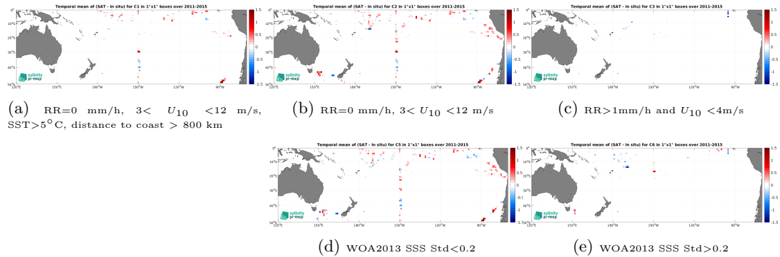
Figure 12: Temporal mean gridded over spatial boxes of size 1^\circ \times 1^\circ of \Delta\text{SSS} (Aquarius SSS L2 CAP v5 (JPL) - TSG (SAMOS)) for 5 different subdatasets corresponding to:RR=0 mm/h, 3 < U_{10} < 12 m/s, SST >5^\circ\text{C} , distance to coast > 800 km (a), RR=0 mm/h, 3 < U_{10} < 12 m/s (b), RR >1 mm/h and U_{10} < 4 m/s (c), WOA2013 SSS Std <0.2 (d), WOA2013 SSS Std >0.2 (e).
