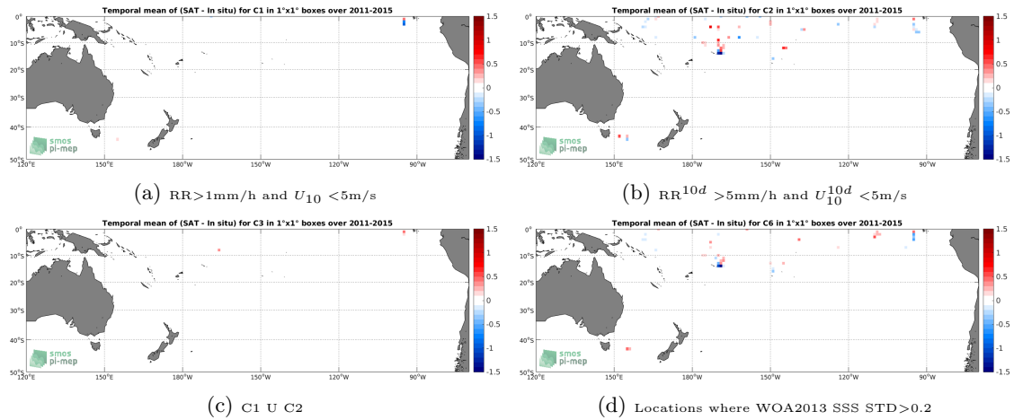
Figure 12: Temporal mean gridded over spatial boxes of size 1^\circ \times 1^\circ of \Delta SSS (Aquarius-L2-JPL-V5 - TSG-SAMOS) for 4 different subdatasets corresponding to: RR > 1\text{mm/h} and U_{10} < 5\text{m/s} (a), RR^{10d} > 5\text{mm/h} and U_{10}^{10d} < 5\text{m/s} (b), C1 U C2 (c), Locations where WOA2013 SSS STD > 0.2 (d).
