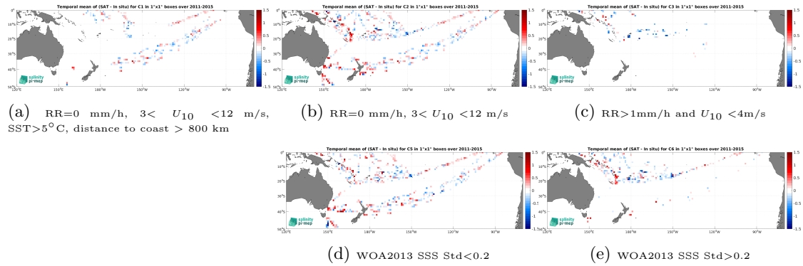
Figure 12: Temporal mean gridded over spatial boxes of size 1^\circ \times 1^\circ of \Delta\text{SSS} (Aquarius SSS L2 CAP v5 (JPL) - TSG (LEGOS-DM)) for 5 different subdatasets corresponding to:RR=0 mm/h, 3 < U_{10} < 12 m/s, SST >5^\circ\text{C} , distance to coast > 800 km (a), RR=0 mm/h, 3 < U_{10} < 12 m/s (b), RR >1 mm/h and U_{10} < 4 m/s (c), WOA2013 SSS Std <0.2 (d), WOA2013 SSS Std >0.2 (e).
