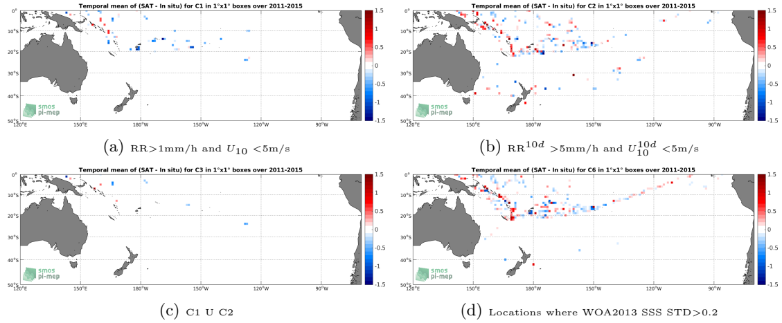
Figure 12: Temporal mean gridded over spatial boxes of size 1^\circ \times 1^\circ of \Delta SSS (Aquarius-L2-JPL-V5 - TSG-LEGOS-DM) for 4 different subdatasets corresponding to: RR > 1\text{mm/h} and U_{10} < 5\text{m/s} (a), RR^{10d} > 5\text{mm/h} and U_{10}^{10d} < 5\text{m/s} (b), C1 U C2 (c), Locations where WOA2013 SSS STD > 0.2 (d).
