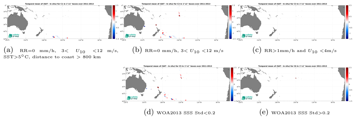
Figure 14: Temporal mean gridded over spatial boxes of size 1^\circ \times 1^\circ of \Delta SSS (Aquarius SSS L2 CAP v5 (JPL) - TSG (GOSUD-Sailing-ship)) for 5 different subdatasets corresponding to:RR=0 mm/h, 3 < U_{10} < 12 m/s, SST > 5°C, distance to coast > 800 km (a), RR=0 mm/h, 3 < U_{10} < 12 m/s (b), RR > 1mm/h and U_{10} < 4 m/s (c), WOA2013 SSS Std < 0.2 (d), WOA2013 SSS Std > 0.2 (e).
