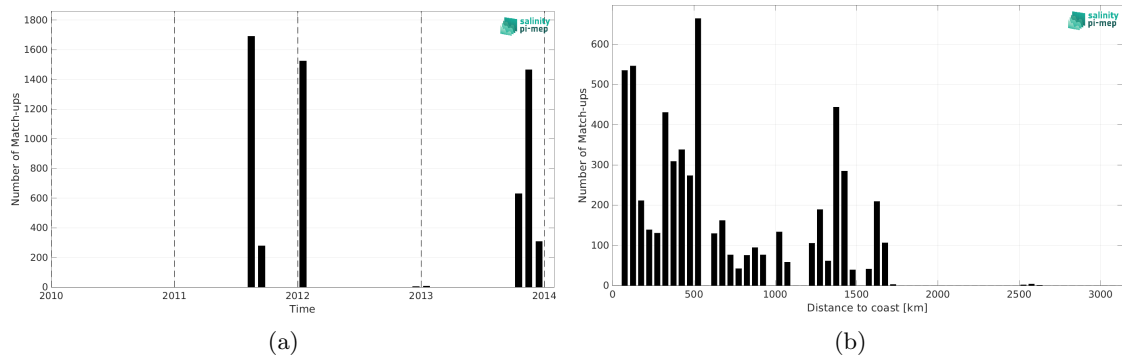
Figure 2: Number of match-ups between TSG (GOSUD-Sailing-ship) and Aquarius SSS L2 CAP v5 (JPL) SSS as a function of time (a) and as function of the distance to coast (b) over the South Pacific Ocean Pi-MEP region and for the full satellite product period.
