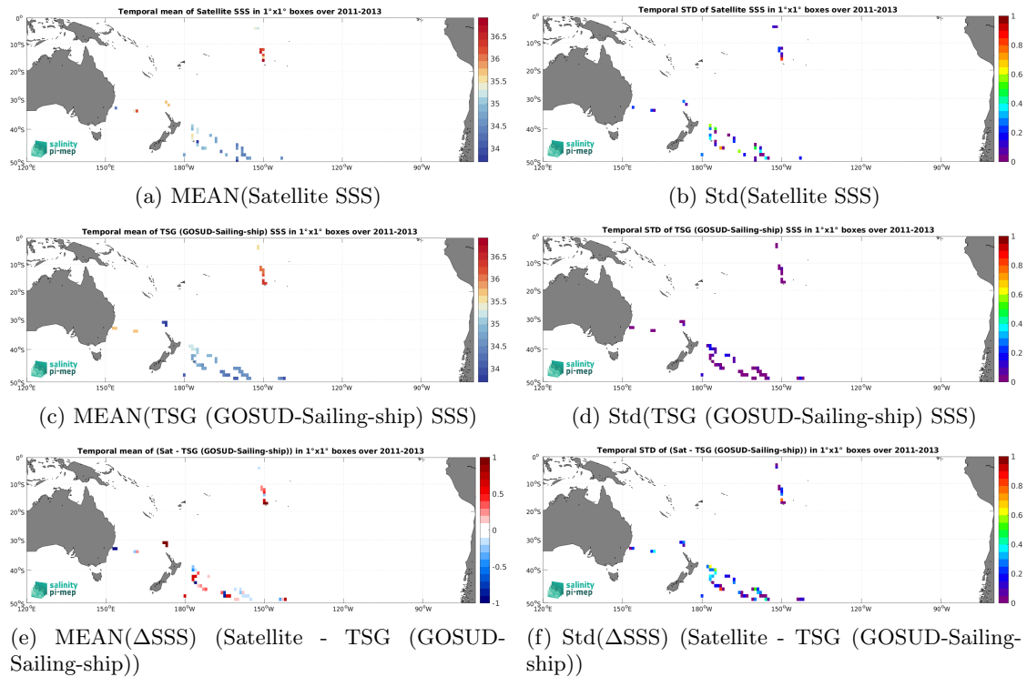
Figure 7: Temporal mean (left) and Std (right) of SSS from Aquarius SSS L2 CAP v5 (JPL) (top), TSG (GOSUD-Sailing-ship) (middle), and of \Delta SSS (Satellite - TSG (GOSUD-Sailing-ship)). Only match-up pairs are used to generate these maps.
