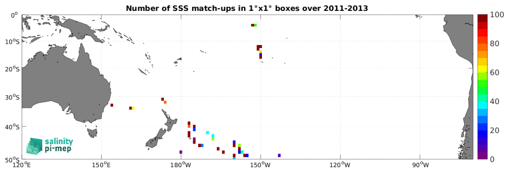
Figure 5: Number of SSS match-ups between TSG (GOSUD-Sailing-ship) SSS and the Aquarius SSS L2 CAP v5 (JPL) SSS product for the South Pacific Ocean Pi-MEP region over 1^\circ \times 1^\circ boxes and for the full satellite product period.
