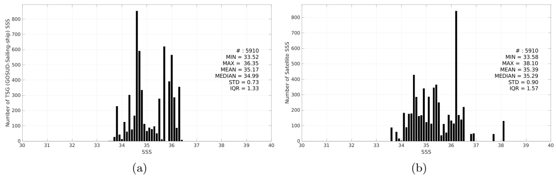
Figure 3: Histograms of SSS from TSG (GOSUD-Sailing-ship) (a) and Aquarius SSS L2 CAP v5 (JPL) (b) considering all match-up pairs per bins of 0.1 over the South Pacific Ocean Pi-MEP region and for the full satellite product period.
