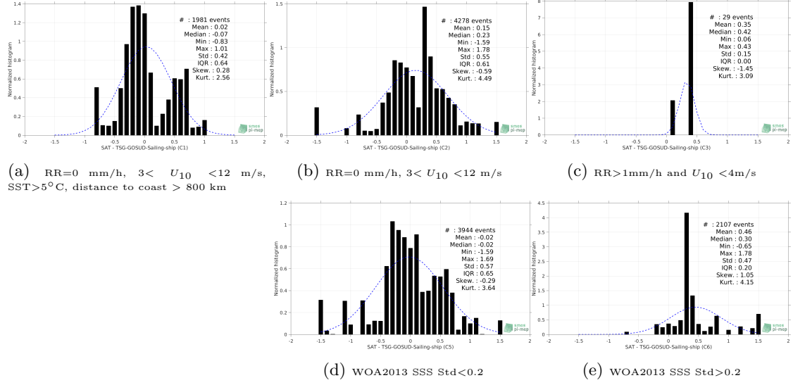
Figure 13: Normalized histogram of \Delta\text{SSS} (Aquarius-L2-JPL-V5 - TSG-GOSUD-Sailing-ship) for 5 different subdatasets corresponding to: RR=0 mm/h, 3 < U_{10} < 12 m/s, SST > 5^\circ\text{C} , distance to coast > 800 km (a), RR=0 mm/h, 3 < U_{10} < 12 m/s (b), RR > 1\text{mm/h} and U_{10} < 4\text{m/s} (c), WOA2013 SSS Std < 0.2 (d), WOA2013 SSS Std > 0.2 (e).
