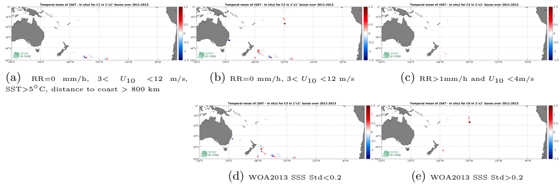
Figure 12: Temporal mean gridded over spatial boxes of size 1^\circ \times 1^\circ of \Delta SSS (Aquarius-L2-JPL-V5 - TSG-GOSUD-Sailing-ship) for 5 different subdatasets corresponding to: RR=0 mm/h, 3 < U_{10} < 12 m/s, SST > 5^\circ\text{C} , distance to coast > 800 km (a), RR=0 mm/h, 3 < U_{10} < 12 m/s (b), RR > 1 mm/h and U_{10} < 4 m/s (c), WOA2013 SSS Std < 0.2 (d), WOA2013 SSS Std > 0.2 (e).
