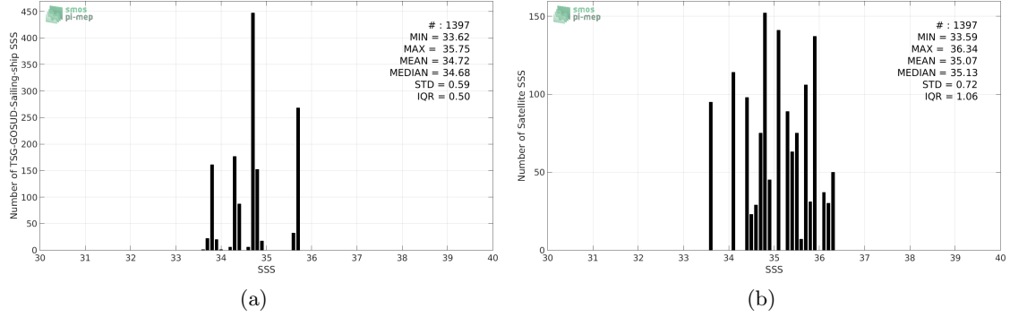
Figure 2: Histograms of SSS from TSG-GOSUD-Sailing-ship (a) and Aquarius-L2-JPL-V5 (b) considering all match-up pairs per bins of 0.1 over the South Pacific Ocean Pi-MEP region and for the full satellite product period.
