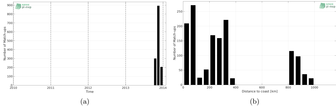
Figure 1: Number of match-ups between TSG-GOSUD-Sailing-ship and Aquarius-L2-JPL-V5 SSS as a function of time (a) and as function of the distance to coast (b) over the South Pacific Ocean Pi-MEP region and for the full satellite product period.
