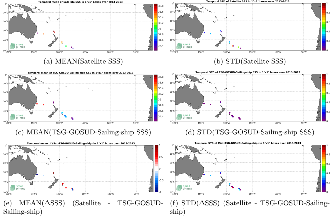
Figure 6: Temporal mean (left) and STD (right) of SSS from Aquarius-L2-JPL-V5 (top), TSG-GOSUD-Sailing-ship (middle), and of \Delta SSS (Satellite - TSG-GOSUD-Sailing-ship). Only match-up pairs are used to generate these maps.
