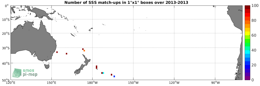
Figure 4: Number of SSS match-ups between TSG-GOSUD-Sailing-ship SSS and the Aquarius-L2-JPL-V5 SSS product for the South Pacific Ocean Pi-MEP region over 1^\circ \times 1^\circ boxes and for the full satellite product period.
