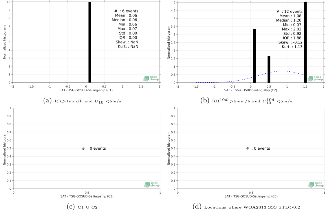
Figure 13: Normalized histogram of \Delta\text{SSS} (Aquarius-L2-JPL-V5 - TSG-GOSUD-Sailing-ship) for 6 different subdatasets corresponding to: RR > 1\text{mm/h} and U_{10} < 5\text{m/s} (a), RR^{10d} > 5\text{mm/h} and U_{10}^{10d} < 5\text{m/s} (b), C1 U C2 (c), Locations where WOA2013 SSS STD > 0.2 (d).
