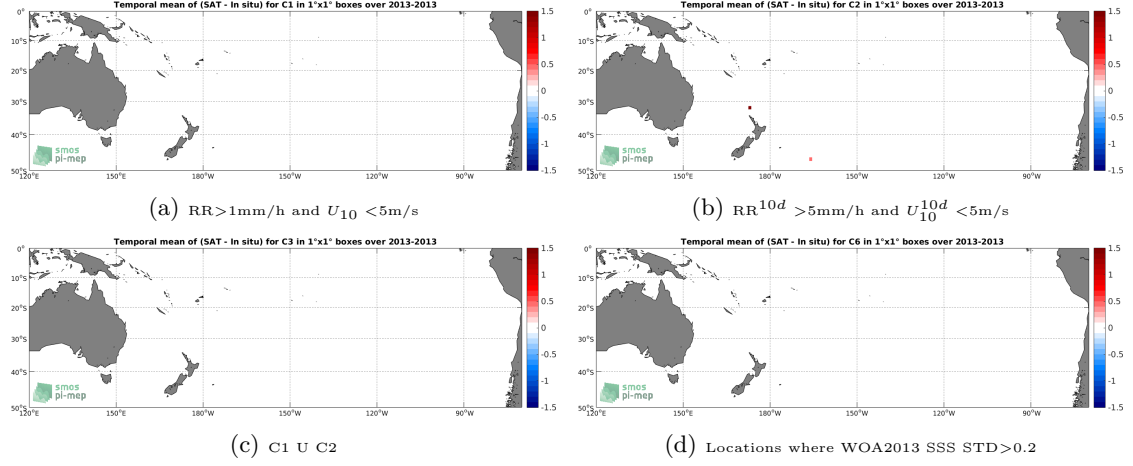
Figure 12: Temporal mean gridded over spatial boxes of size 1^\circ \times 1^\circ of \Delta SSS (Aquarius-L2-JPL-V5 - TSG-GOSUD-Sailing-ship) for 4 different subdatasets corresponding to: RR > 1\text{mm/h} and U_{10} < 5\text{m/s} (a), RR^{10d} > 5\text{mm/h} and U_{10}^{10d} < 5\text{m/s} (b), C1 U C2 (c), Locations where WOA2013 SSS STD > 0.2 (d).
