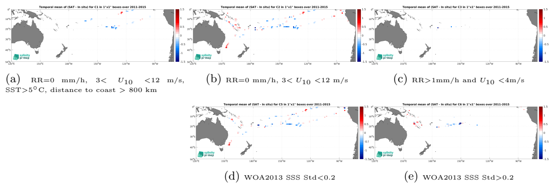
Figure 14: Temporal mean gridded over spatial boxes of size 1^\circ \times 1^\circ of \Delta SSS (Aquarius SSS L2 CAP v5 (JPL) - TSG (GOSUD-Research-vessel)) for 5 different subdatasets corresponding to:RR=0 mm/h, 3 < U_{10} < 12 m/s, SST >5^\circ\text{C} , distance to coast > 800 km (a), RR=0 mm/h, 3 < U_{10} < 12 m/s (b), RR >1 mm/h and U_{10} < 4 m/s (c), WOA2013 SSS Std <0.2 (d), WOA2013 SSS Std >0.2 (e).
