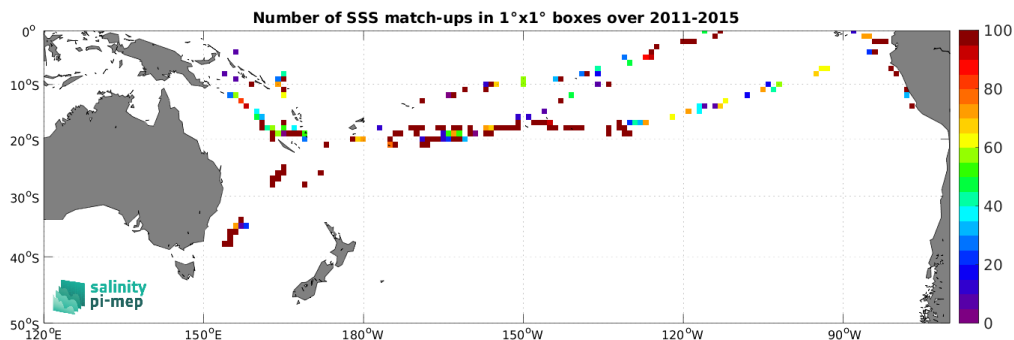
Figure 5: Number of SSS match-ups between TSG (GOSUD-Research-vessel) SSS and the Aquarius SSS L2 CAP v5 (JPL) SSS product for the South Pacific Ocean Pi-MEP region over 1^\circ \times 1^\circ boxes and for the full satellite product period.
