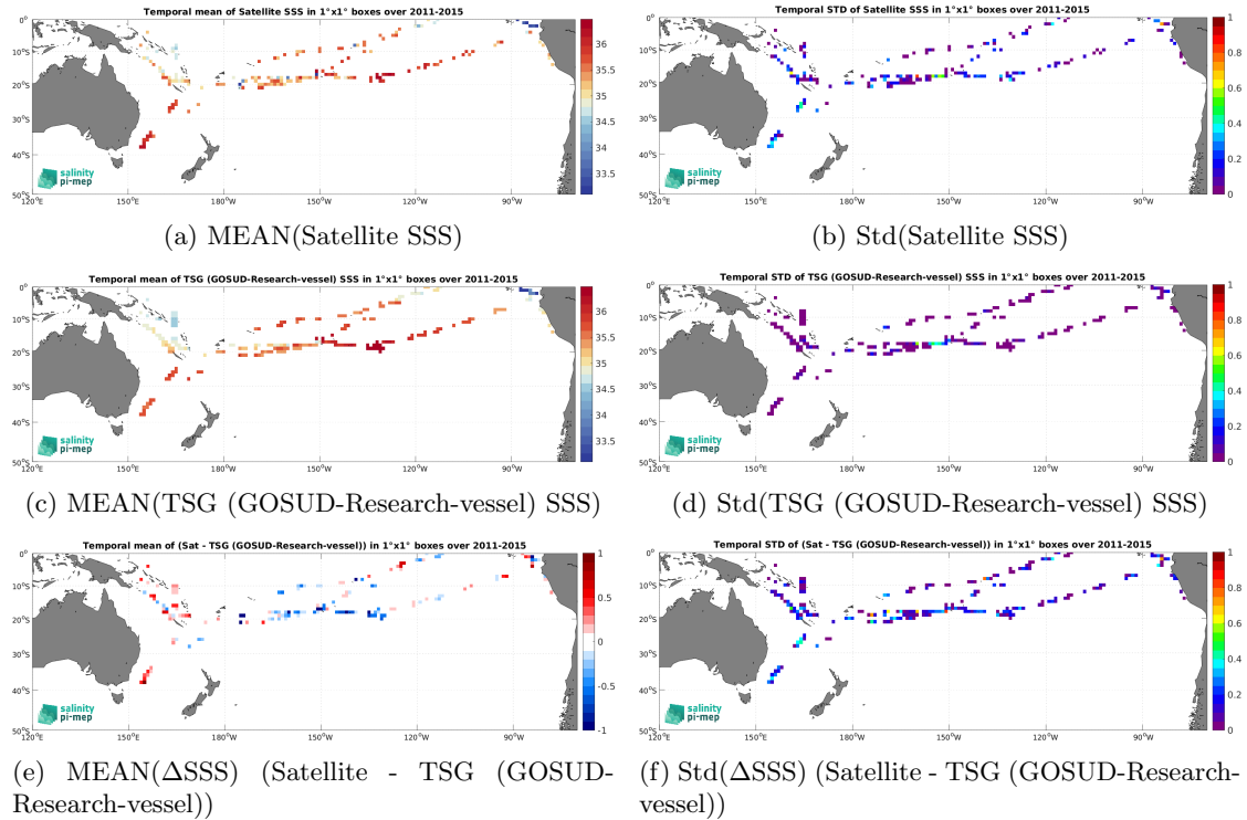
Figure 7: Temporal mean (left) and Std (right) of SSS from Aquarius SSS L2 CAP v5 (JPL) (top), TSG (GOSUD-Research-vessel) (middle), and of \Delta SSS (Satellite - TSG (GOSUD-Research-vessel)). Only match-up pairs are used to generate these maps.
