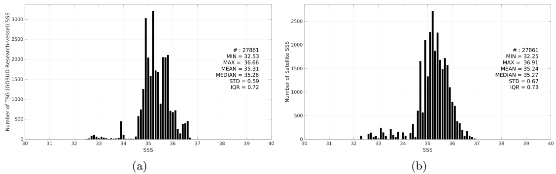
Figure 3: Histograms of SSS from TSG (GOSUD-Research-vessel) (a) and Aquarius SSS L2 CAP v5 (JPL) (b) considering all match-up pairs per bins of 0.1 over the South Pacific Ocean Pi-MEP region and for the full satellite product period.
