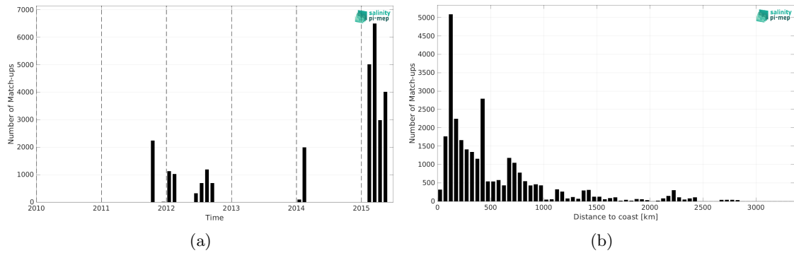
Figure 2: Number of match-ups between TSG (GOSUD-Research-vessel) and Aquarius SSS L2 CAP v5 (JPL) SSS as a function of time (a) and as function of the distance to coast (b) over the South Pacific Ocean Pi-MEP region and for the full satellite product period.
