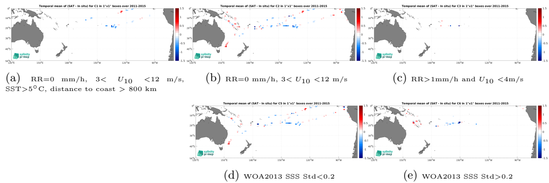
Figure 14: Temporal mean gridded over spatial boxes of size 1^\circ \times 1^\circ of \Delta\text{SSS} (Aquarius SSS L2 CAP v5 (JPL) - TSG (GOSUD-Research-vessel)) for 5 different subdatasets corresponding to:RR=0 mm/h, 3 < U_{10} < 12 m/s, SST>5°C, distance to coast > 800 km (a), RR=0 mm/h, 3 < U_{10} < 12 m/s (b), RR>1mm/h and U_{10} < 4 m/s (c), WOA2013 SSS Std<0.2 (d), WOA2013 SSS Std>0.2 (e).
