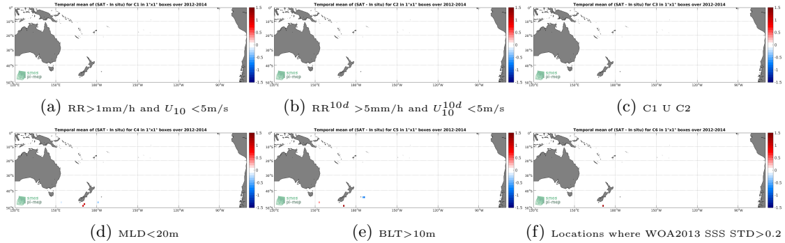
Figure 12: Temporal mean gridded over spatial boxes of size 1^\circ \times 1^\circ of \Delta SSS (Aquarius-L2-JPL-V5 - Sea mammals) for 6 different subdatasets corresponding to: RR > 1\text{mm/h} and U_{10} < 5\text{m/s} (a), RR^{10d} > 5\text{mm/h} and U_{10}^{10d} < 5\text{m/s} (b), C1 U C2 (c), MLD < 20\text{m} (d), BLT > 10\text{m} (e), Locations where WOA2013 SSS STD > 0.2 (f).
