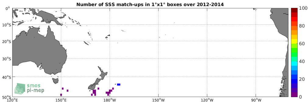
Figure 4: Number of SSS match-ups between Sea mammals SSS and the Aquarius-L2-JPL-V5 SSS product for the South Pacific Ocean Pi-MEP region over 1^\circ \times 1^\circ boxes and for the full satellite product period.
