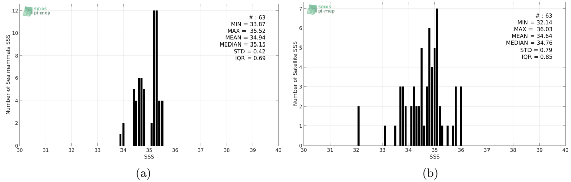
Figure 2: Histograms of SSS from Sea mammals (a) and Aquarius-L2-JPL-V5 (b) considering all match-up pairs per bins of 0.1 over the South Pacific Ocean Pi-MEP region and for the full satellite product period.
