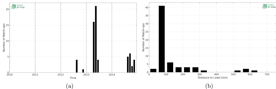
Figure 1: Number of match-ups between Sea mammals and Aquarius-L2-JPL-V5 SSS as a function of time (a) and as function of the distance to coast (b) over the South Pacific Ocean Pi-MEP region and for the full satellite product period.
