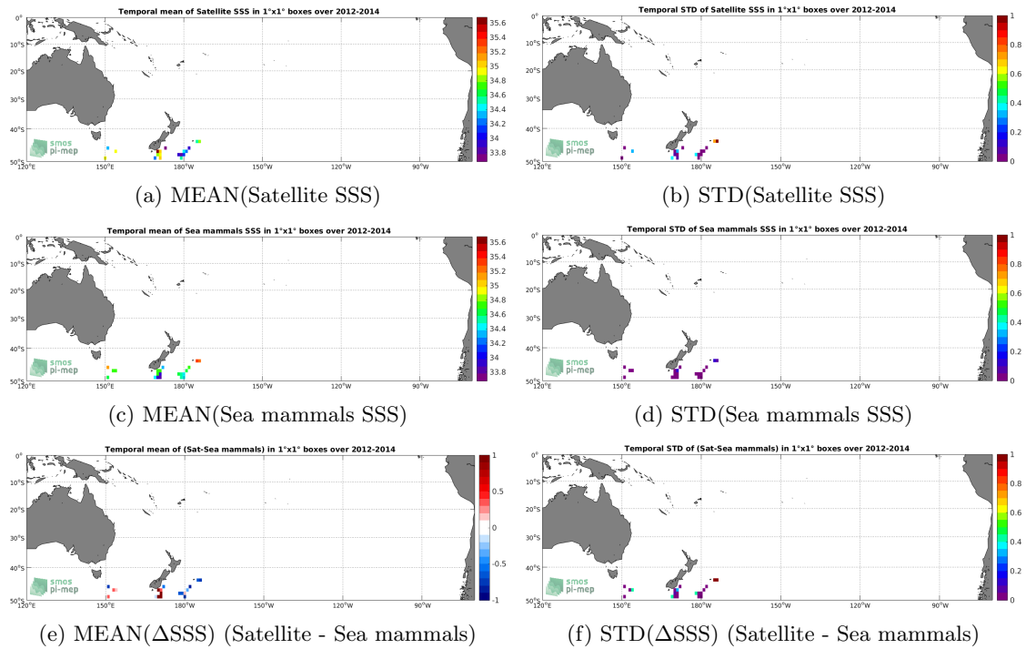
Figure 6: Temporal mean (left) and STD (right) of SSS from Aquarius-L2-JPL-V5 (top), Sea mammals (middle), and of \Delta SSS (Satellite - Sea mammals). Only match-up pairs are used to generate these maps.
