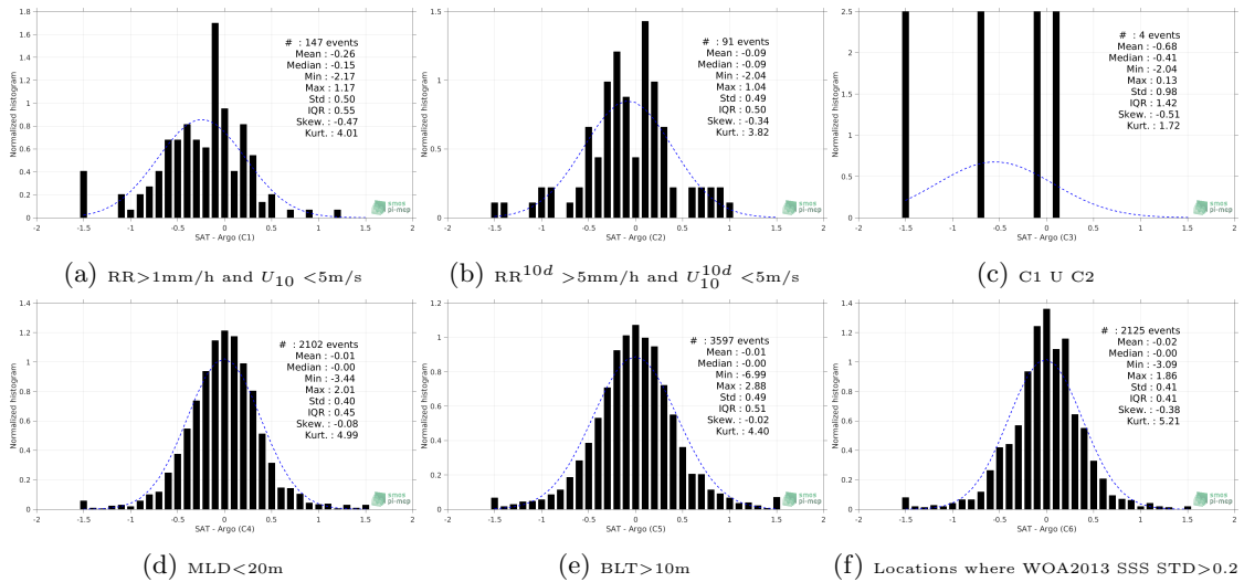
Figure 13: Normalized histogram of \Delta SSS (Aquarius-L2-JPL-V5 - Argo) for 6 different subdatasets corresponding to: RR>1mm/h and U_{10} <5m/s (a), RR^{10d} >5mm/h and U_{10}^{10d} <5m/s (b), C1 U C2 (c),MLD<20m (d),BLT>10m (e),Locations where WOA2013 SSS STD>0.2 (f).
