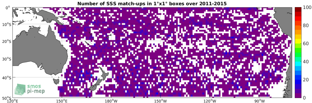
Figure 4: Number of SSS match-ups between Argo SSS and the Aquarius-L2-JPL-V5 SSS product for the South Pacific Ocean Pi-MEP region over 1^\circ \times 1^\circ boxes and for the full satellite product period.
