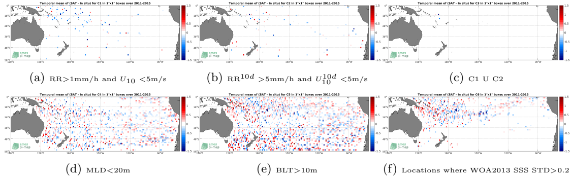
Figure 12: Temporal mean gridded over spatial boxes of size 1°x1° of \Delta SSS (Aquarius-L2-JPL-V5 - Argo) for 6 different subdatasets corresponding to:RR>1mm/h and U_{10} <5m/s (a), RR^{10d} >5mm/h and U_{10}^{10d} <5m/s (b), C1 U C2 (c),MLD<20m (d),BLT>10m (e),Locations where WOA2013 SSS STD>0.2 (f).
