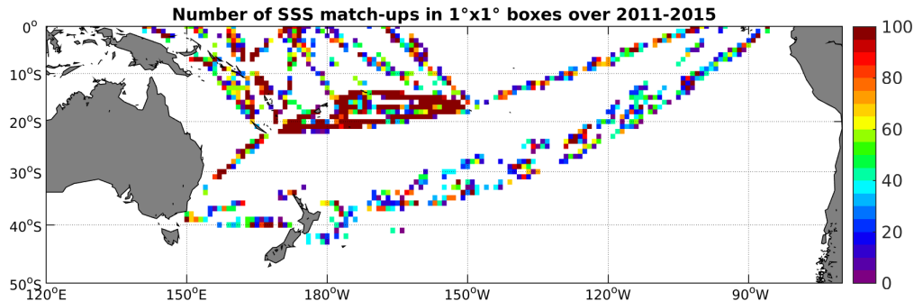
Figure 4: Number of SSS match-ups between TSG-LEGOS-DM SSS and the AQUARIUS-L2-JPL-V4 SSS product for the South Pacific Ocean Pi-MEP region over 1^\circ \times 1^\circ boxes and for the full satellite product period.
