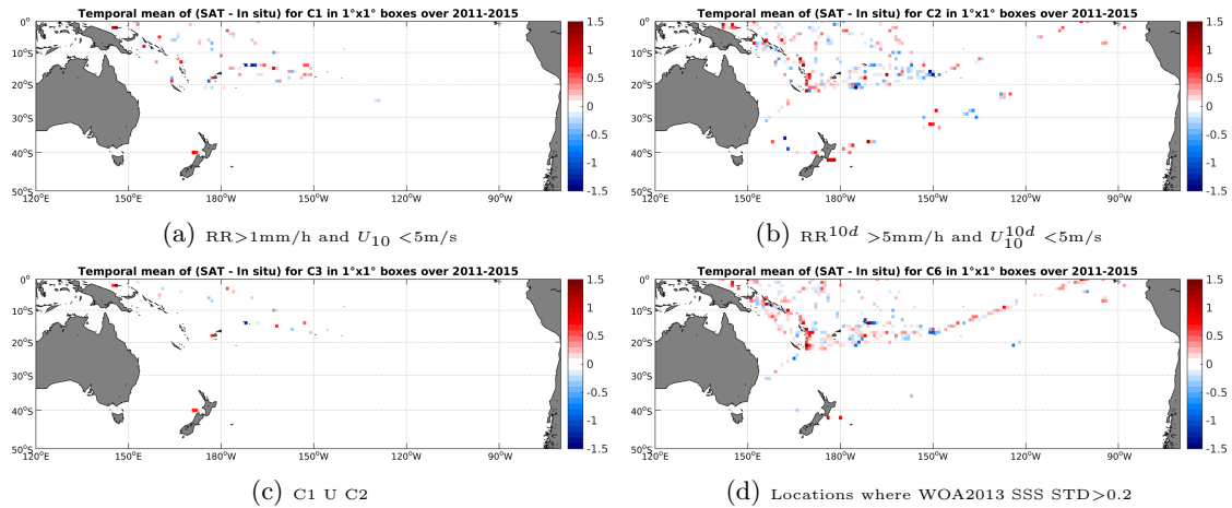
Figure 12: Temporal mean gridded over spatial boxes of size 1^\circ \times 1^\circ of \Delta SSS (AQUARIUS-L2-JPL-V4 - TSG-LEGOS-DM) for 4 different subdatasets corresponding to:RR >1 mm/h and U_{10} < 5 m/s (a), RR^{10d} > 5 mm/h and U_{10}^{10d} < 5 m/s (b), C1 U C2 (c),Locations where WOA2013 SSS STD >0.2 (d).
