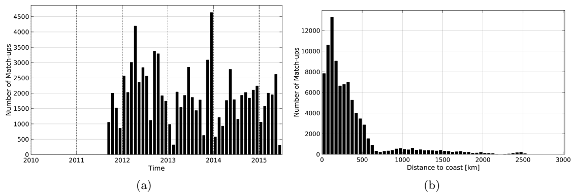
Figure 1: Number of match-ups between TSG-LEGOS-DM and AQUARIUS-L2-JPL-V4 SSS as a function of time (a) and as function of the distance to coast (b) over the South Pacific Ocean Pi-MEP region and for the full satellite product period.
