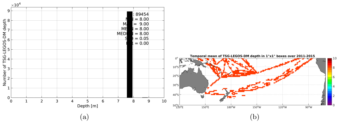
Figure 3: Histograms of the depth of the upper level SSS measurements from TSG-LEGOS-DM in the Match-up DataBase for the South Pacific Ocean Pi-MEP region (a) and temporal mean spatial distribution of pressure of the in situ SSS data over 1°x1° boxes and for the full satellite product period (b).
