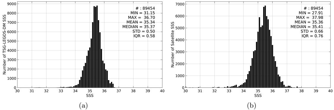
Figure 2: Histograms of SSS from TSG-LEGOS-DM (a) and AQUARIUS-L2-JPL-V4 (b) considering all match-up pairs per bins of 0.1 over the South Pacific Ocean Pi-MEP region and for the full satellite product period.
