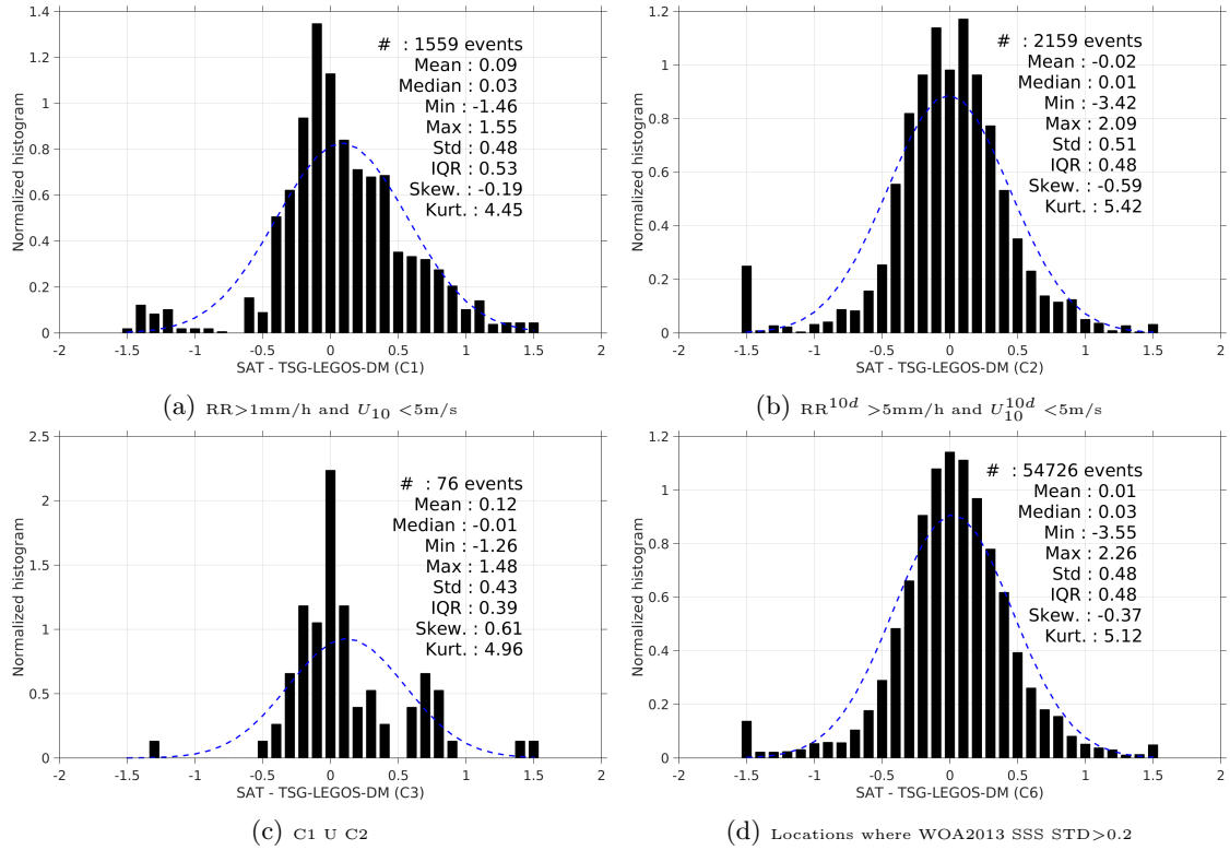
Figure 13: Normalized histogram of \Delta\text{SSS} (AQUARIUS-L2-JPL-V4 - TSG-LEGOS-DM) for 6 different subdatasets corresponding to: RR > 1mm/h and U_{10} < 5\text{m/s} (a), RR^{10d} > 5\text{mm/h} and U_{10}^{10d} < 5\text{m/s} (b), C1 U C2 (c), Locations where WOA2013 SSS STD > 0.2 (d).
