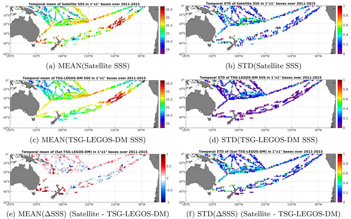
Figure 6: Temporal mean (left) and STD (right) of SSS from AQUARIUS-L2-JPL-V4 (top), TSG-LEGOS-DM (middle), and of \Delta SSS (Satellite - TSG-LEGOS-DM). Only match-up pairs are used to generate these maps.
