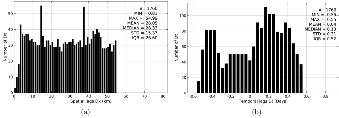
Figure 5: Histograms of the spatial (a) and temporal (b) lags between the time of the TSG-GOSUD-Sailing-ship measurements and the date of the corresponding AQUARIUS-L2-JPL-V4 SSS product.
