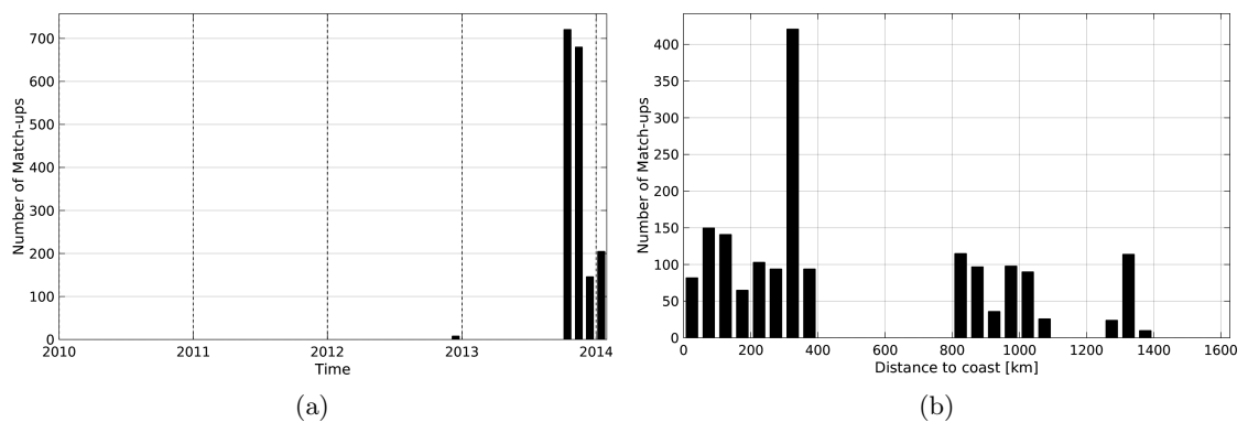
Figure 1: Number of match-ups between TSG-GOSUD-Sailing-ship and AQUARIUS-L2-JPL-V4 SSS as a function of time (a) and as function of the distance to coast (b) over the South Pacific Ocean Pi-MEP region and for the full satellite product period.
