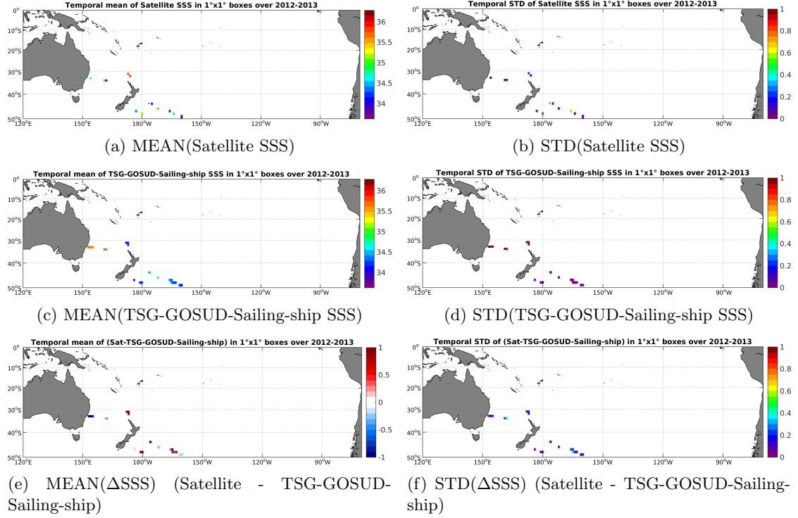
Figure 6: Temporal mean (left) and STD (right) of SSS from AQUARIUS-L2-JPL-V4 (top), TSG-GOSUD-Sailing-ship (middle), and of \Delta SSS (Satellite - TSG-GOSUD-Sailing-ship). Only match-up pairs are used to generate these maps.
