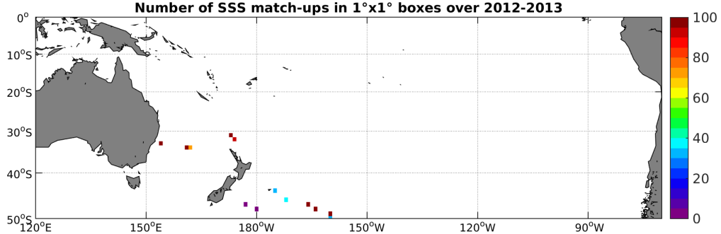
Figure 4: Number of SSS match-ups between TSG-GOSUD-Sailing-ship SSS and the AQUARIUS-L2-JPL-V4 SSS product for the South Pacific Ocean Pi-MEP region over 1^\circ \times 1^\circ boxes and for the full satellite product period.
