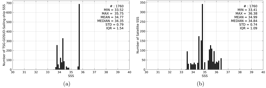
Figure 2: Histograms of SSS from TSG-GOSUD-Sailing-ship (a) and AQUARIUS-L2-JPL-V4 (b) considering all match-up pairs per bins of 0.1 over the South Pacific Ocean Pi-MEP region and for the full satellite product period.
