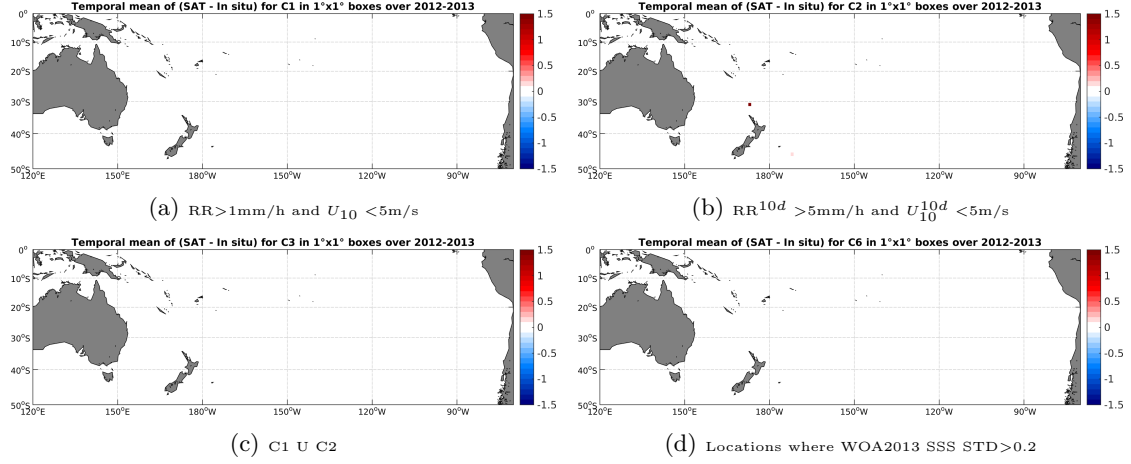
Figure 12: Temporal mean gridded over spatial boxes of size 1^\circ \times 1^\circ of \Delta SSS (AQUARIUS-L2-JPL-V4 - TSG-GOSUD-Sailing-ship) for 4 different subdatasets corresponding to: RR > 1 mm/h and U_{10} < 5 m/s (a), RR^{10d} > 5 mm/h and U_{10}^{10d} < 5 m/s (b), C1 U C2 (c), Locations where WOA2013 SSS STD > 0.2 (d).
