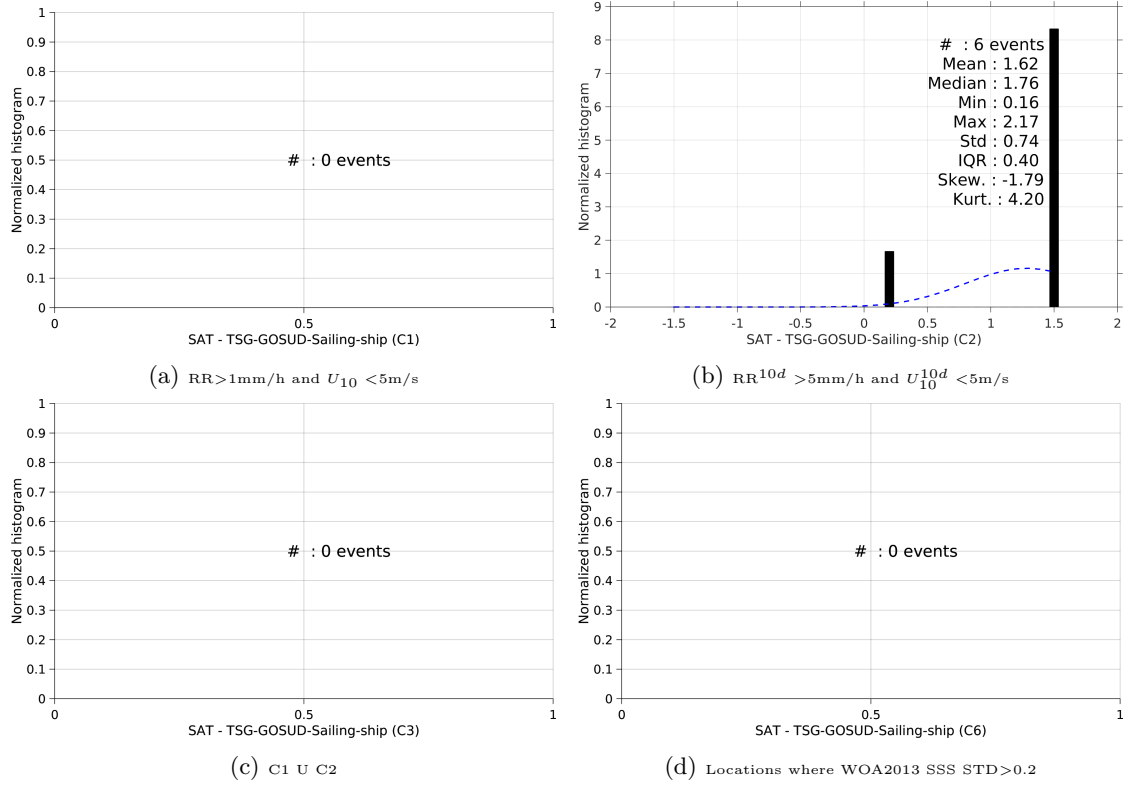
Figure 13: Normalized histogram of \Delta SSS (AQUARIUS-L2-JPL-V4 - TSG-GOSUD-Sailing-ship) for 6 different subdatasets corresponding to: RR > 1\text{mm/h} and U_{10} < 5\text{m/s} (a), RR^{10d} > 5\text{mm/h} and U_{10}^{10d} < 5\text{m/s} (b), C1 U C2 (c), Locations where WOA2013 SSS STD > 0.2 (d).
