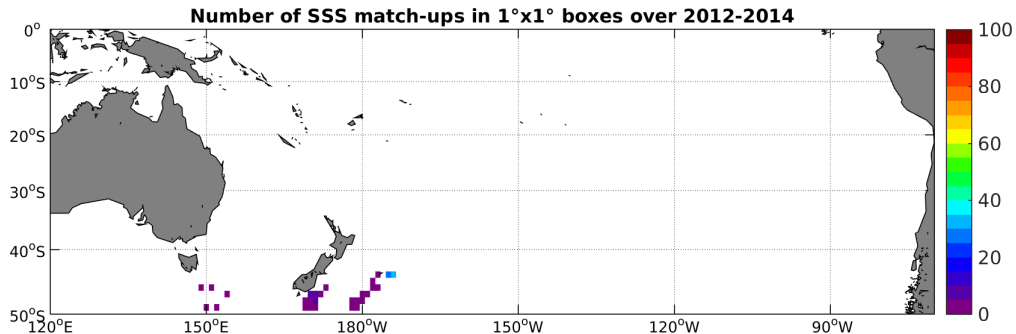
Figure 4: Number of SSS match-ups between Sea mammals SSS and the AQUARIUS-L2-JPL-V4 SSS product for the South Pacific Ocean Pi-MEP region over 1^\circ \times 1^\circ boxes and for the full satellite product period.
