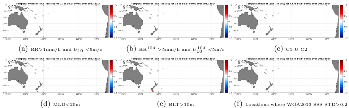
Figure 12: Temporal mean gridded over spatial boxes of size 1^\circ \times 1^\circ of \Delta SSS (AQUARIUS-L2-JPL-V4 - Sea mammals) for 6 different subdatasets corresponding to: RR > 1\text{mm/h} and U_{10} < 5\text{m/s} (a), RR^{10d} > 5\text{mm/h} and U_{10}^{10d} < 5\text{m/s} (b), C1 U C2 (c), MLD < 20\text{m} (d), BLT > 10\text{m} (e), Locations where WOA2013 SSS STD > 0.2 (f).
