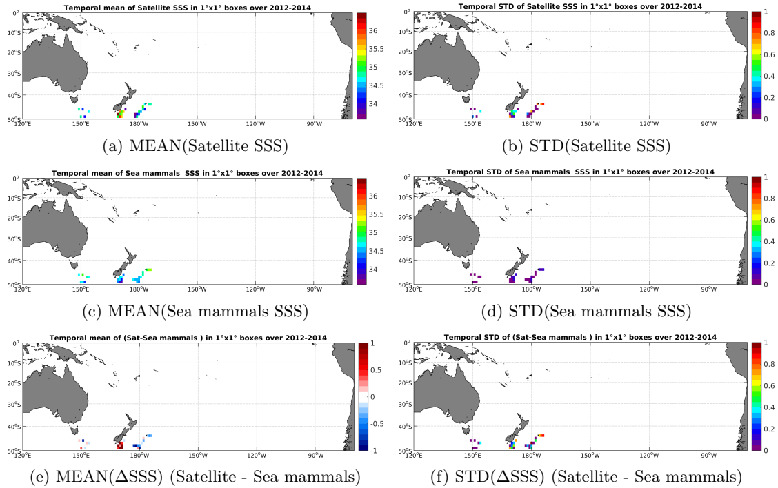
Figure 6: Temporal mean (left) and STD (right) of SSS from AQUARIUS-L2-JPL-V4 (top), Sea mammals (middle), and of \Delta SSS (Satellite - Sea mammals). Only match-up pairs are used to generate these maps.
