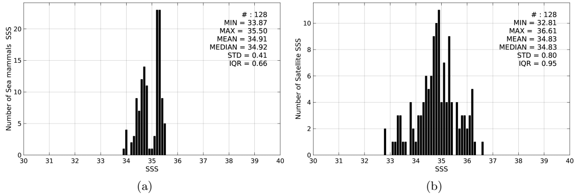
Figure 2: Histograms of SSS from Sea mammals (a) and AQUARIUS-L2-JPL-V4 (b) considering all match-up pairs per bins of 0.1 over the South Pacific Ocean Pi-MEP region and for the full satellite product period.
