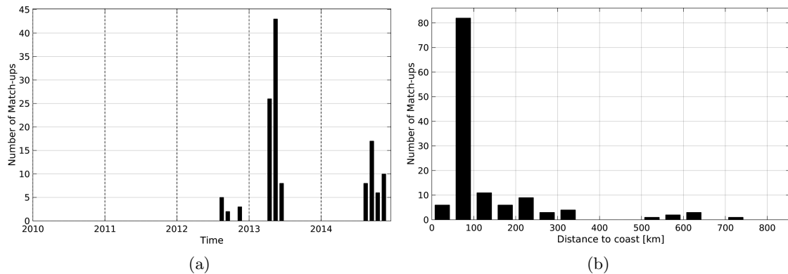
Figure 1: Number of match-ups between Sea mammals and AQUARIUS-L2-JPL-V4 SSS as a function of time (a) and as function of the distance to coast (b) over the South Pacific Ocean Pi-MEP region and for the full satellite product period.
