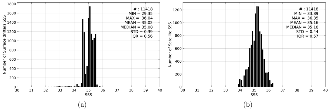
Figure 2: Histograms of SSS from Surface drifters (a) and AQUARIUS-L2-JPL-V4 (b) considering all match-up pairs per bins of 0.1 over the South Pacific Ocean Pi-MEP region and for the full satellite product period.
