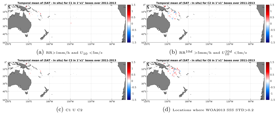
Figure 11: Temporal mean gridded over spatial boxes of size 1^\circ \times 1^\circ of \Delta SSS (AQUARIUS-L2-JPL-V4 - Surface drifters) for 4 different subdatasets corresponding to:RR >1 mm/h and U_{10} < 5 m/s (a), RR 10d > 5 mm/h and U_{10}^{10d} < 5 m/s (b), C1 U C2 (c),Locations where WOA2013 SSS STD >0.2 (d).
