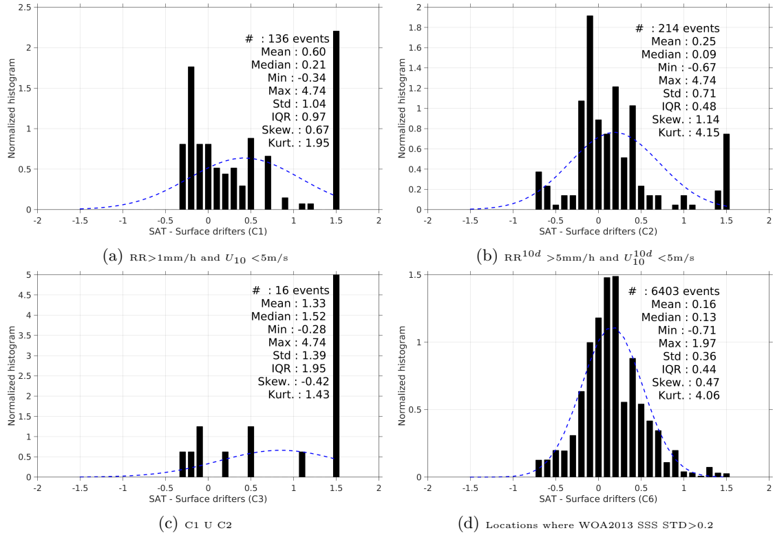
Figure 12: Normalized histogram of \Delta\text{SSS} (AQUARIUS-L2-JPL-V4 - Surface drifters) for 6 different subdatasets corresponding to: RR > 1mm/h and U_{10} < 5\text{m/s} (a), RR^{10d} > 5\text{mm/h} and U_{10}^{10d} < 5\text{m/s} (b), C1 U C2 (c), Locations where WOA2013 SSS STD > 0.2 (d).
