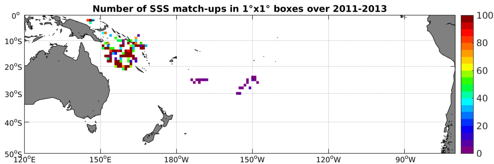
Figure 3: Number of SSS match-ups between Surface drifters SSS and the AQUARIUS-L2-JPL-V4 SSS product for the South Pacific Ocean Pi-MEP region over 1°x1° boxes and for the full satellite product period.
