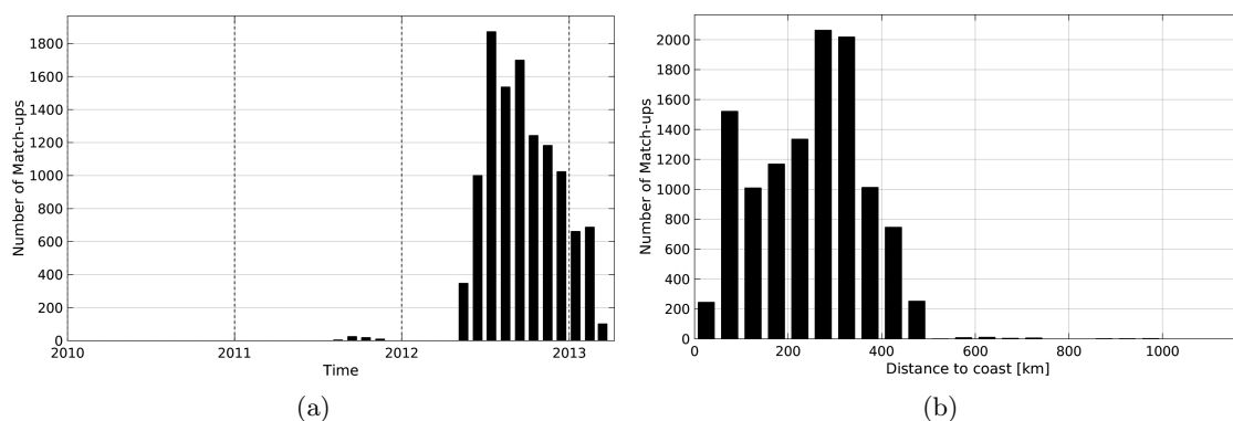
Figure 1: Number of match-ups between Surface drifters and AQUARIUS-L2-JPL-V4 SSS as a function of time (a) and as function of the distance to coast (b) over the South Pacific Ocean Pi-MEP region and for the full satellite product period.
