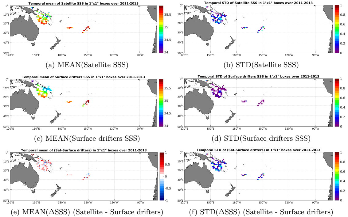
Figure 5: Temporal mean (left) and STD (right) of SSS from AQUARIUS-L2-JPL-V4 (top), Surface drifters (middle), and of \Delta SSS (Satellite - Surface drifters). Only match-up pairs are used to generate these maps.
