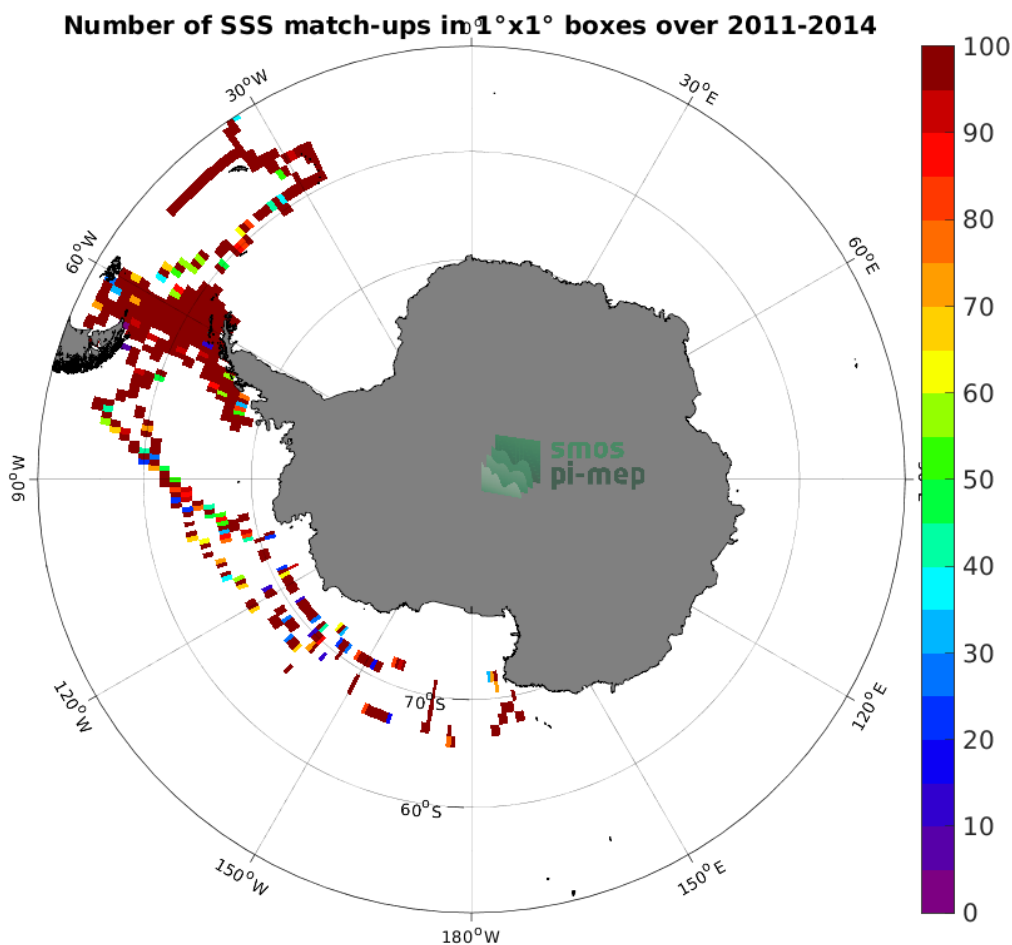
Figure 4: Number of SSS match-ups between TSG (SAMOS) SSS and the SMOS and SMAP SSS L4 OI v1 - 7 Days (LOPS) SSS product for the Southern Ocean Pi-MEP region over 1^\circ \times 1^\circ boxes and for the full satellite product period.
