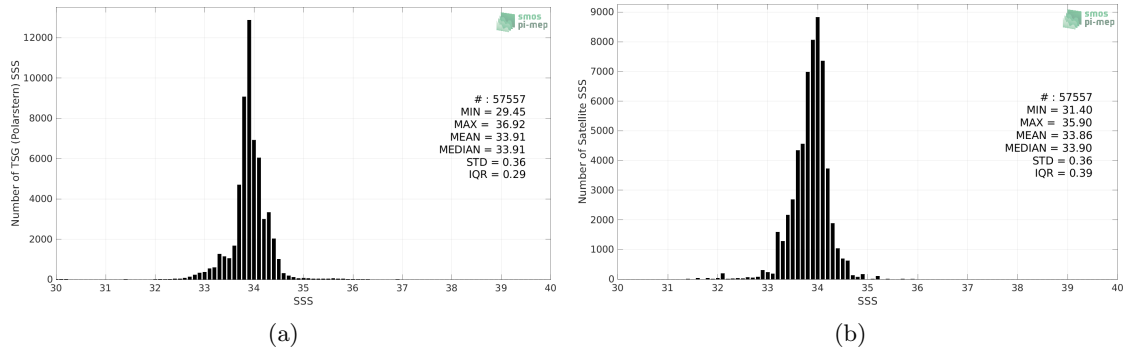
Figure 2: Histograms of SSS from TSG (Polarstern) (a) and SMOS and SMAP SSS L4 OI v1 - 7 Days (LOPS) (b) considering all match-up pairs per bins of 0.1 over the Southern Ocean Pi-MEP region and for the full satellite product period.
