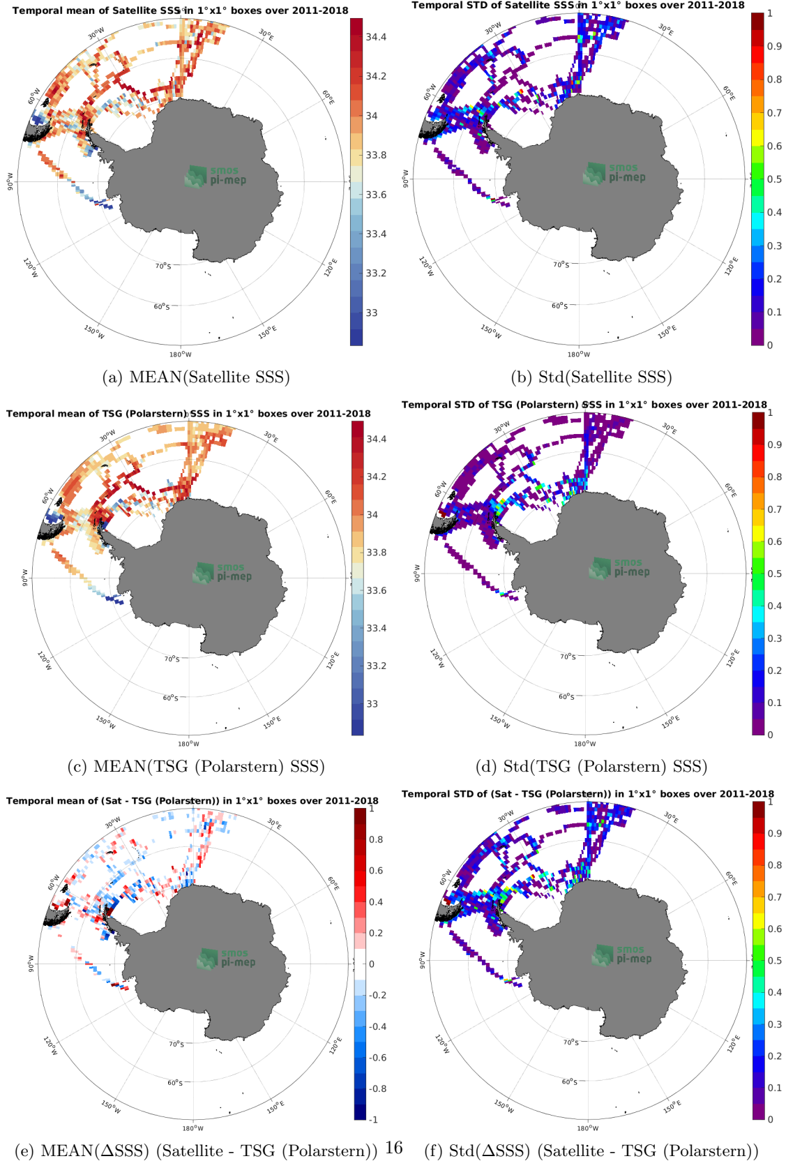
Figure 6: Temporal mean (left) and Std (right) of SSS from SMOS and SMAP SSS L4 OI v1 - 7 Days (LOPS) (top), TSG (Polarstern) (middle), and of \Delta SSS (Satellite - TSG (Polarstern)). Only match-up pairs are used to generate these maps.
