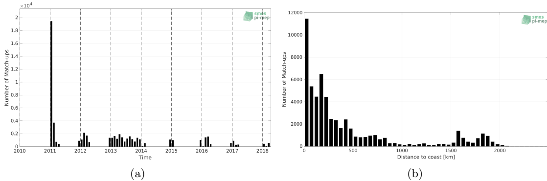
Figure 1: Number of match-ups between TSG (Polarstern) and SMOS and SMAP SSS L4 OI v1 - 7 Days (LOPS) SSS as a function of time (a) and as function of the distance to coast (b) over the Southern Ocean Pi-MEP region and for the full satellite product period.
