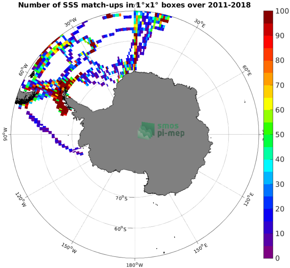
Figure 4: Number of SSS match-ups between TSG (Polarstern) SSS and the SMOS and SMAP SSS L4 OI v1 - 7 Days (LOPS) SSS product for the Southern Ocean Pi-MEP region over 1^\circ \times 1^\circ boxes and for the full satellite product period.
