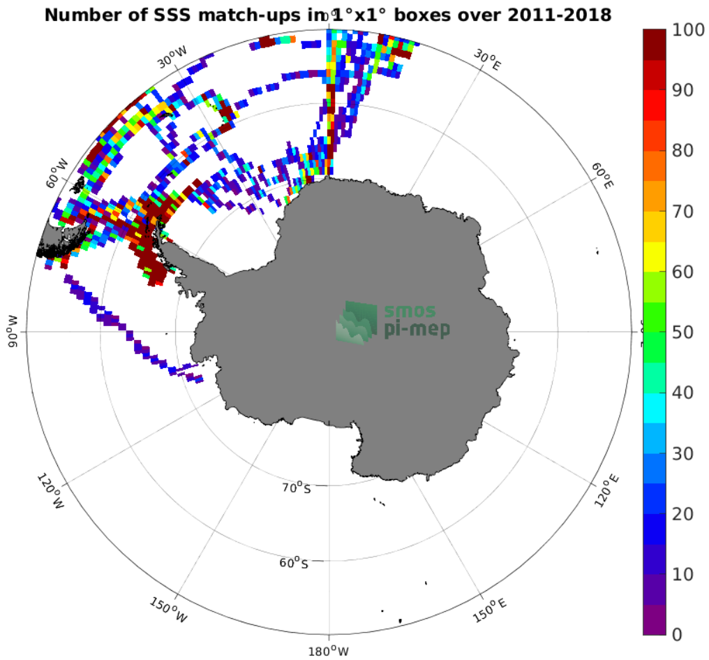
Figure 4: Number of SSS match-ups between TSG (Polarstern) SSS and the SMOS and SMAP SSS L4 OI v1 - 7 Days (LOPS) SSS product for the Southern Ocean Pi-MEP region over 1^\circ \times 1^\circ boxes and for the full satellite product period.
