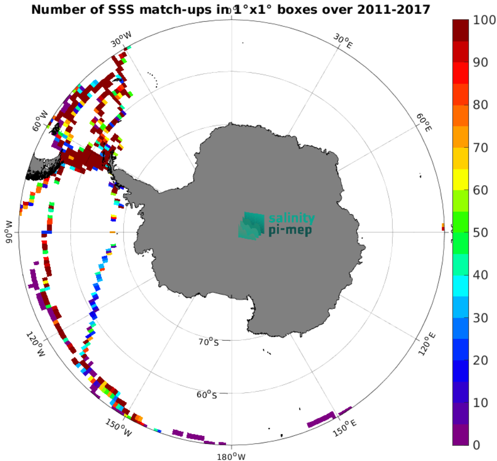
Figure 4: Number of SSS match-ups between TSG (GOSUD-Sailing-ship) SSS and the SMOS and SMAP SSS L4 OI v1 - 7 Days (LOPS) SSS product for the Southern Ocean Pi-MEP region over 1^\circ \times 1^\circ boxes and for the full satellite product period.
