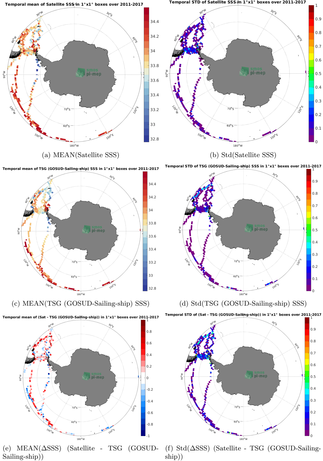
Figure 6: Temporal mean (left) and Std (right) of SSS from SMOS and SMAP SSS L4 OI v1 - 7 Days (LOPS) (top), TSG (GOSUD-Sailing-ship) (middle), and of \Delta SSS (Satellite - TSG (GOSUD-Sailing-ship)). Only match-up pairs are used to generate these maps.
