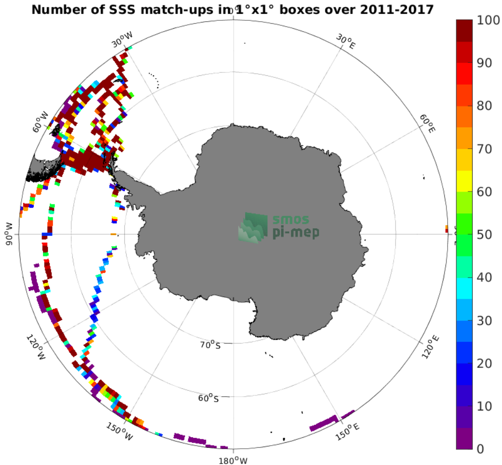
Figure 4: Number of SSS match-ups between TSG (GOSUD-Sailing-ship) SSS and the SMOS and SMAP SSS L4 OI v1 - 7 Days (LOPS) SSS product for the Southern Ocean Pi-MEP region over 1^\circ \times 1^\circ boxes and for the full satellite product period.
