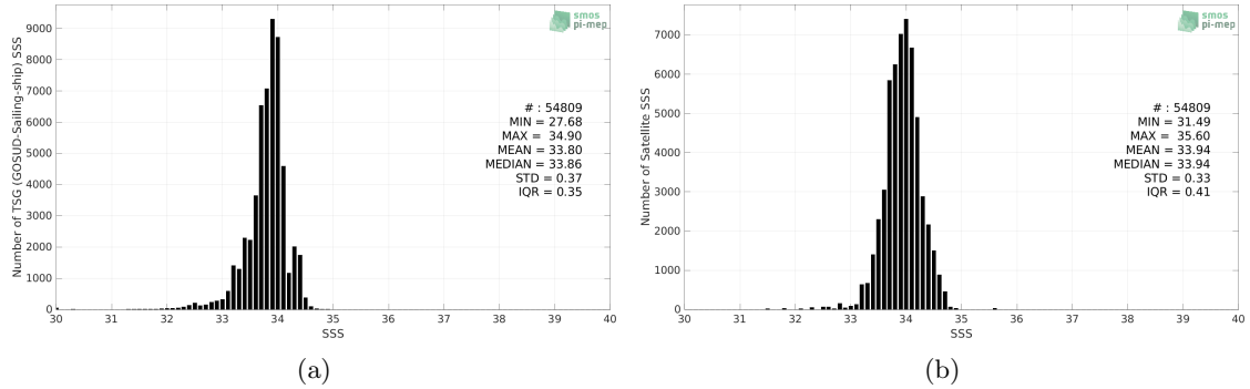
Figure 2: Histograms of SSS from TSG (GOSUD-Sailing-ship) (a) and SMOS and SMAP SSS L4 OI v1 - 7 Days (LOPS) (b) considering all match-up pairs per bins of 0.1 over the Southern Ocean Pi-MEP region and for the full satellite product period.
