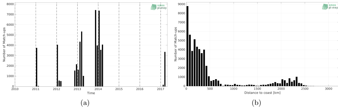
Figure 1: Number of match-ups between TSG (GOSUD-Sailing-ship) and SMOS and SMAP SSS L4 OI v1 - 7 Days (LOPS) SSS as a function of time (a) and as function of the distance to coast (b) over the Southern Ocean Pi-MEP region and for the full satellite product period.
