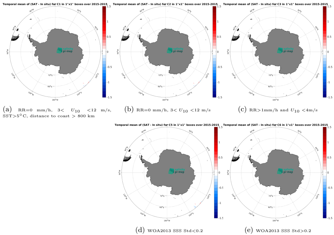
Figure 12: Temporal mean gridded over spatial boxes of size 1^\circ \times 1^\circ of \Delta\text{SSS} (SMOS and SMAP SSS L4 OI v1 - 7 Days (LOPS) - TSG (GOSUD-Research-vessel)) for 5 different subdatasets corresponding to: RR=0 mm/h, 3 < U_{10} < 12 m/s, SST > 5^\circ\text{C} , distance to coast > 800 km (a), RR=0 mm/h, 3 < U_{10} < 12 m/s (b), RR > 1 mm/h and U_{10} < 4 m/s (c), WOA2013 SSS Std < 0.2 (d), WOA2013 SSS Std > 0.2 (e).
