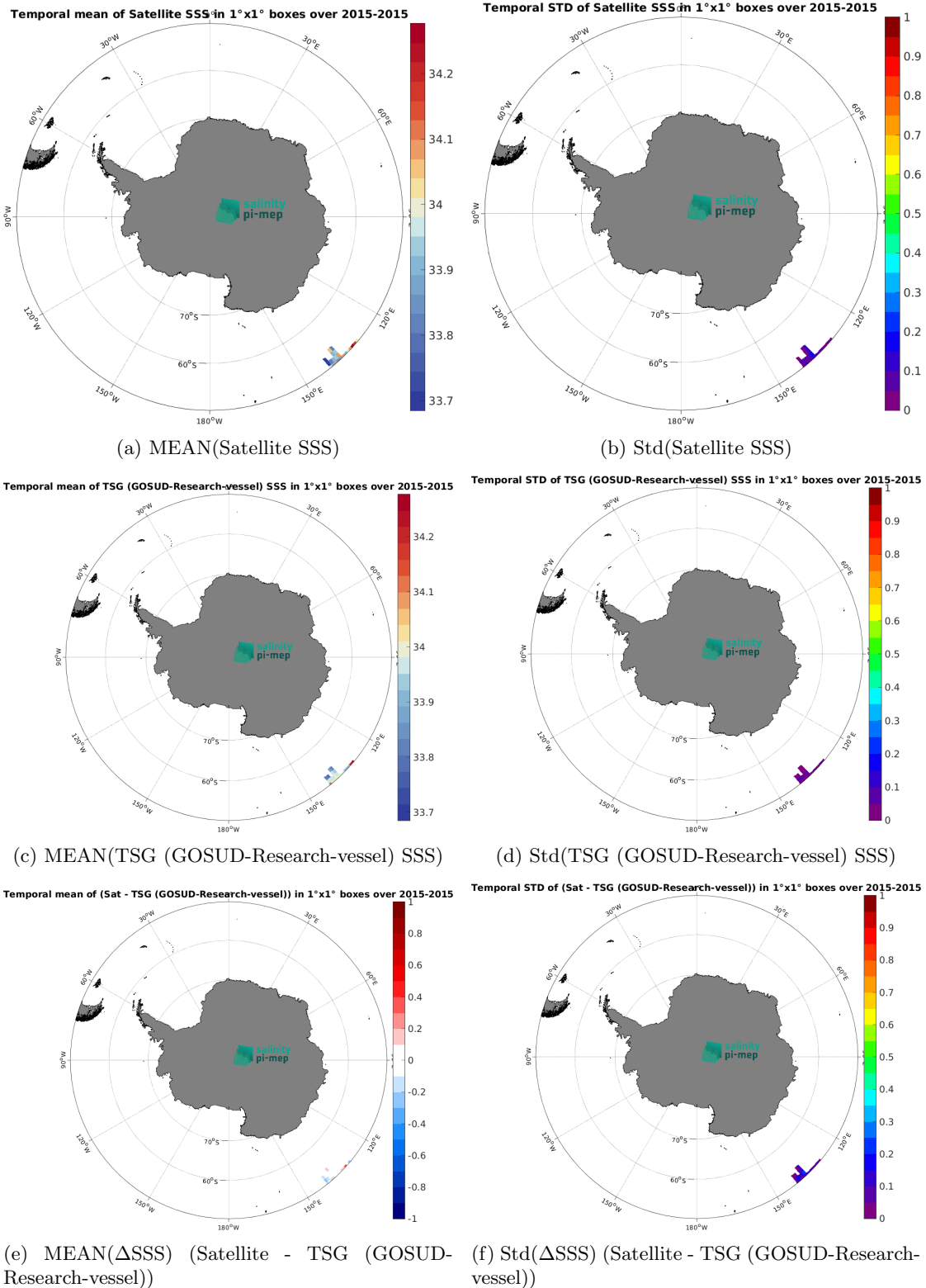
Figure 6: Temporal mean (left) and Std (right) of SSS from SMOS and SMAP SSS L4 OI v1 - 7 Days (LOPS) (top), TSG (GOSUD-Research-vessel) (middle), and of \Delta SSS (Satellite - TSG (GOSUD-Research-vessel)). Only match-up pairs are used to generate these maps.
