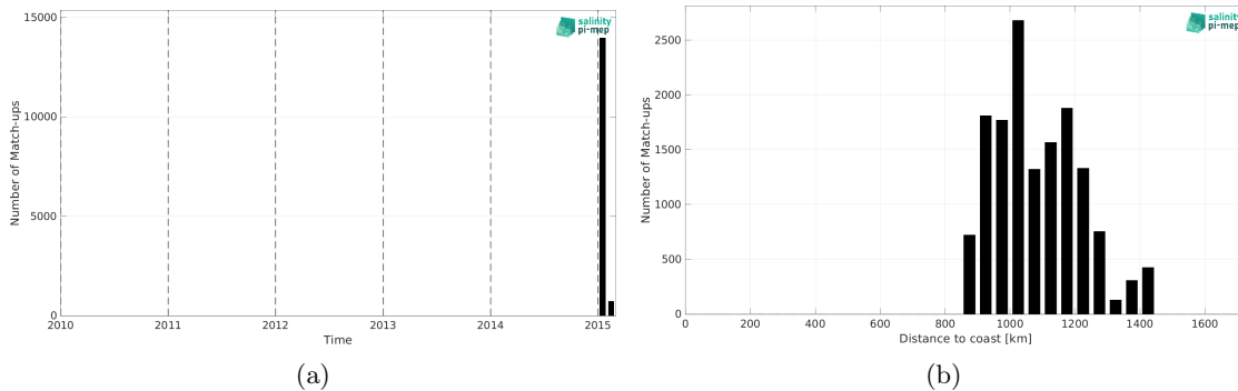
Figure 1: Number of match-ups between TSG (GOSUD-Research-vessel) and SMOS and SMAP SSS L4 OI v1 - 7 Days (LOPS) SSS as a function of time (a) and as function of the distance to coast (b) over the Southern Ocean Pi-MEP region and for the full satellite product period.
