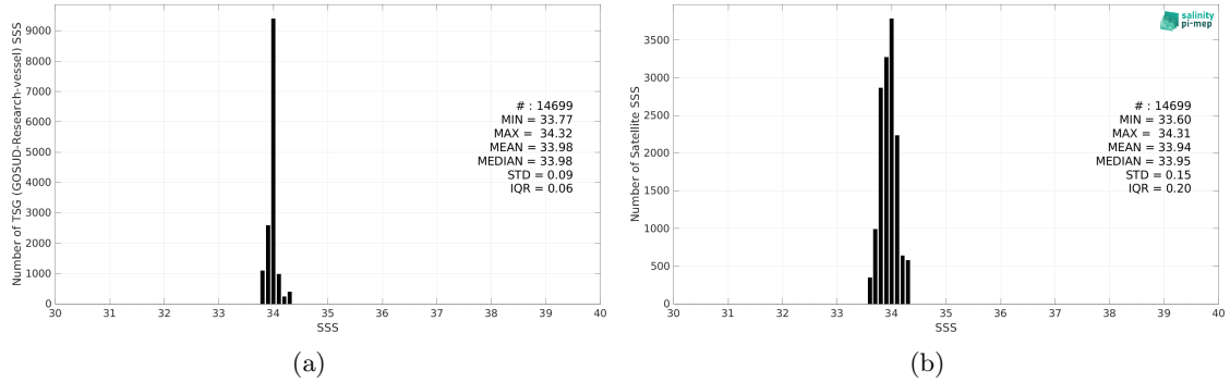
Figure 2: Histograms of SSS from TSG (GOSUD-Research-vessel) (a) and SMOS and SMAP SSS L4 OI v1 - 7 Days (LOPS) (b) considering all match-up pairs per bins of 0.1 over the Southern Ocean Pi-MEP region and for the full satellite product period.
