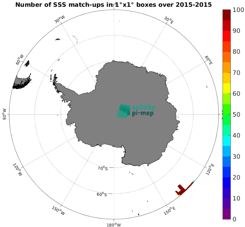
Figure 4: Number of SSS match-ups between TSG (GOSUD-Research-vessel) SSS and the SMOS and SMAP SSS L4 OI v1 - 7 Days (LOPS) SSS product for the Southern Ocean Pi-MEP region over 1^\circ \times 1^\circ boxes and for the full satellite product period.
