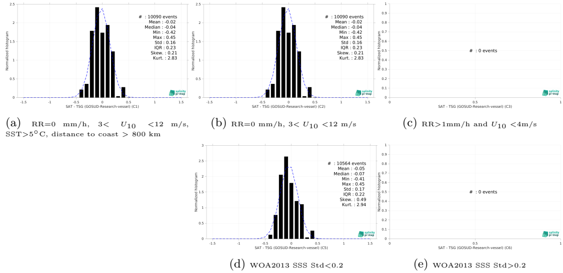
Figure 13: Normalized histogram of \Delta\text{SSS} (SMOS and SMAP SSS L4 OI v1 - 7 Days (LOPS) - TSG (GOSUD-Research-vessel)) for 5 different subdatasets corresponding to: RR=0 mm/h, 3 < U_{10} < 12 m/s, SST > 5^\circ\text{C} , distance to coast > 800 km (a), RR=0 mm/h, 3 < U_{10} < 12 m/s (b), RR > 1\text{mm/h} and U_{10} < 4\text{m/s} (c), WOA2013 SSS Std < 0.2 (d), WOA2013 SSS Std > 0.2 (e).
