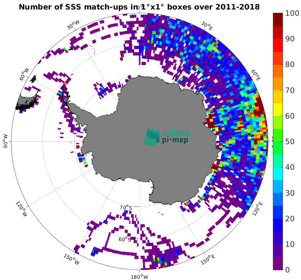
Figure 4: Number of SSS match-ups between Marine mammals SSS and the SMOS and SMAP SSS L4 OI v1 - 7 Days (LOPS) SSS product for the Southern Ocean Pi-MEP region over 1^{\circ} \times 1^{\circ} boxes and for the full satellite product period.
