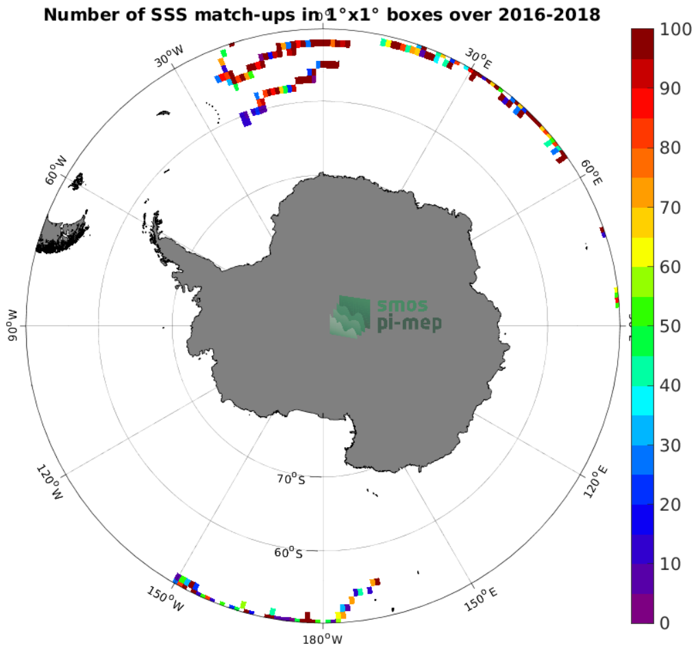
Figure 3: Number of SSS match-ups between Surface drifters SSS and the SMOS and SMAP SSS L4 OI v1 - 7 Days (LOPS) SSS product for the Southern Ocean Pi-MEP region over 1^\circ \times 1^\circ boxes and for the full satellite product period.
