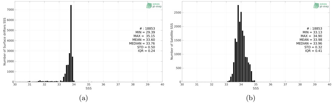
Figure 2: Histograms of SSS from Surface drifters (a) and SMOS and SMAP SSS L4 OI v1 - 7 Days (LOPS) (b) considering all match-up pairs per bins of 0.1 over the Southern Ocean Pi-MEP region and for the full satellite product period.
