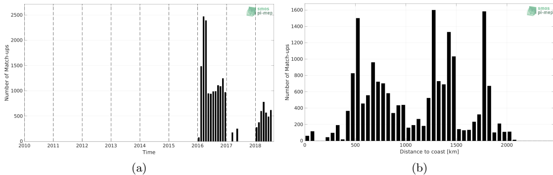
Figure 1: Number of match-ups between Surface drifters and SMOS and SMAP SSS L4 OI v1 - 7 Days (LOPS) SSS as a function of time (a) and as function of the distance to coast (b) over the Southern Ocean Pi-MEP region and for the full satellite product period.
