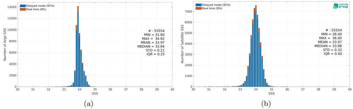
Figure 2: Histograms of SSS from Argo (a) and SMOS and SMAP SSS L4 OI v1 - 7 Days (LOPS) (b) considering all match-up pairs per bins of 0.1 over the Southern Ocean Pi-MEP region and for the full satellite product period.
