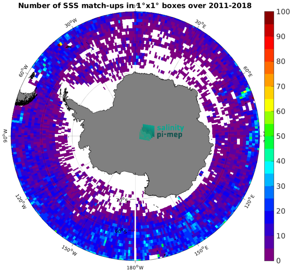
Figure 4: Number of SSS match-ups between Argo SSS and the SMOS and SMAP SSS L4 OI v1 - 7 Days (LOPS) SSS product for the Southern Ocean Pi-MEP region over 1^\circ \times 1^\circ boxes and for the full satellite product period.
