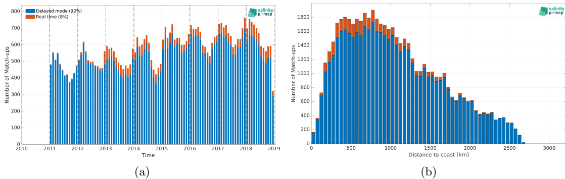
Figure 1: Number of match-ups between Argo and SMOS and SMAP SSS L4 OI v1 - 7 Days (LOPS) SSS as a function of time (a) and as function of the distance to coast (b) over the Southern Ocean Pi-MEP region and for the full satellite product period.
