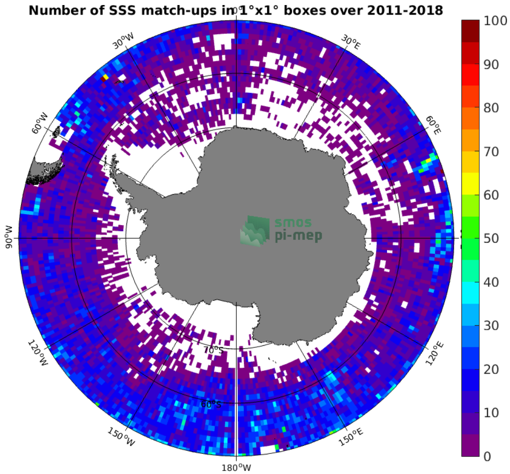
Figure 4: Number of SSS match-ups between Argo SSS and the SMOS and SMAP SSS L4 OI v1 - 7 Days (LOPS) SSS product for the Southern Ocean Pi-MEP region over 1^\circ \times 1^\circ boxes and for the full satellite product period.
