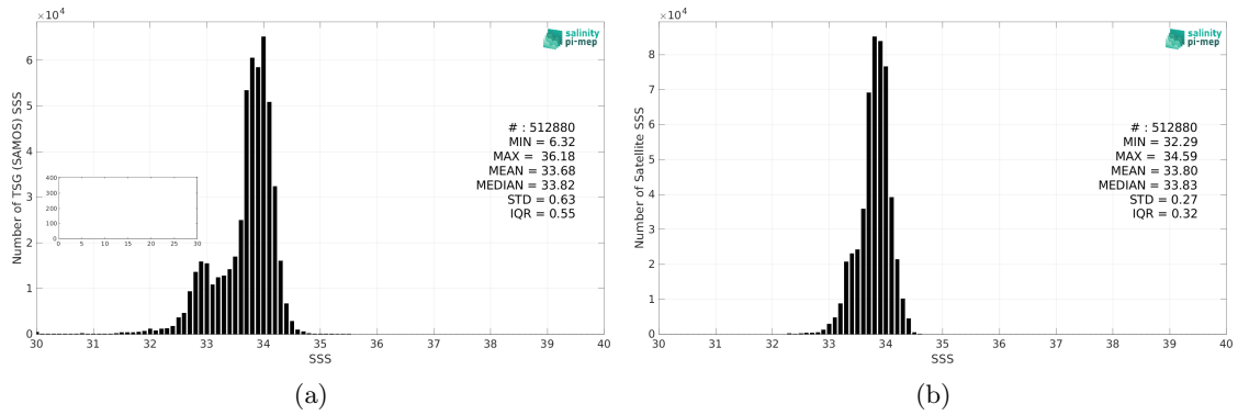
Figure 2: Histograms of SSS from TSG (SAMOS) (a) and SMOS SSS L4 v1 - Weekly (CMEMS-CNR) (b) considering all match-up pairs per bins of 0.1 over the Southern Ocean Pi-MEP region and for the full satellite product period.
