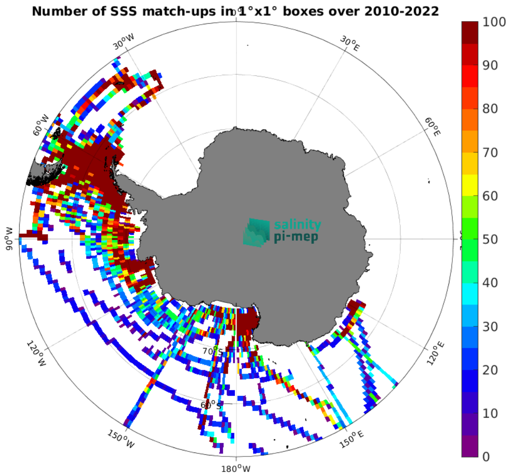
Figure 4: Number of SSS match-ups between TSG (SAMOS) SSS and the SMOS SSS L4 v1 - Weekly (CMEMS-CNR) SSS product for the Southern Ocean Pi-MEP region over 1^\circ \times 1^\circ boxes and for the full satellite product period.
