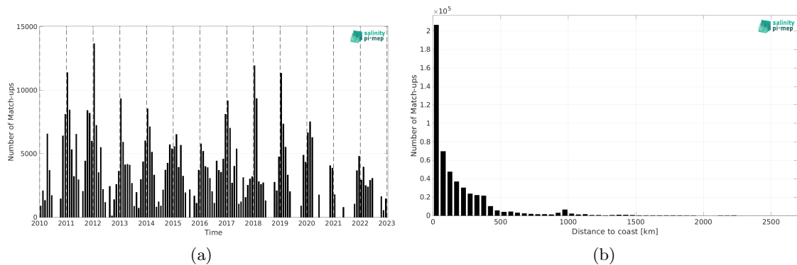
Figure 1: Number of match-ups between TSG (SAMOS) and SMOS SSS L4 v1 - Weekly (CMEMS-CNR) SSS as a function of time (a) and as function of the distance to coast (b) over the Southern Ocean Pi-MEP region and for the full satellite product period.
