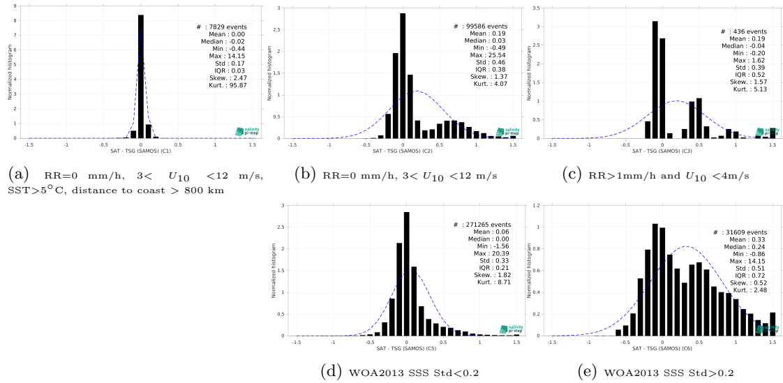
Figure 13: Normalized histogram of \Delta SSS (SMOS SSS L4 v1 - Weekly (CMEMS-CNR) - TSG (SAMOS)) for 5 different subdatasets corresponding to: RR=0 mm/h, 3 < U_{10} < 12 m/s, SST > 5^\circ C , distance to coast > 800 km (a), RR=0 mm/h, 3 < U_{10} < 12 m/s (b), RR > 1 mm/h and U_{10} < 4 m/s (c), WOA2013 SSS Std < 0.2 (d), WOA2013 SSS Std > 0.2 (e).
