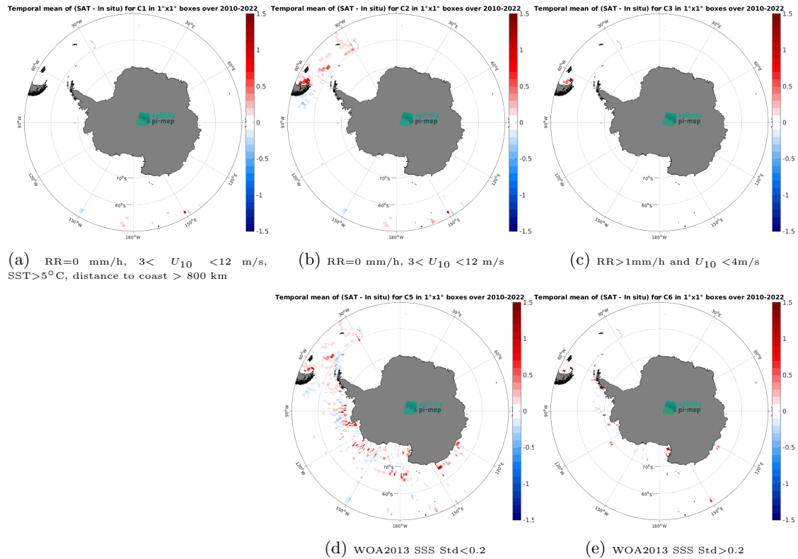
Figure 12: Temporal mean gridded over spatial boxes of size 1^{\circ}\times 1^{\circ} of \Delta\text{SSS} (SMOS SSS L4 v1 - Weekly (CMEMS-CNR) - TSG (SAMOS)) for 5 different subdatasets corresponding to:RR=0 mm/h, 3 < U_{10} < 12 m/s, \text{SST}>5^{\circ}\text{C} , distance to coast > 800 km (a), RR=0 mm/h, 3 < U_{10} < 12 m/s (b), RR >1 mm/h and U_{10} < 4 m/s (c), WOA2013 SSS Std <0.2 (d), WOA2013 SSS Std >0.2 (e).
