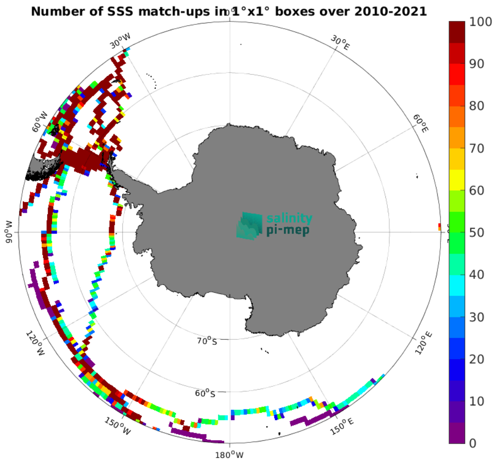
Figure 4: Number of SSS match-ups between TSG (GOSUD-Sailing-ship) SSS and the SMOS SSS L4 v1 - Weekly (CMEMS-CNR) SSS product for the Southern Ocean Pi-MEP region over 1^{\circ} \times 1^{\circ} boxes and for the full satellite product period.
