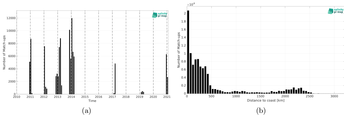
Figure 1: Number of match-ups between TSG (GOSUD-Sailing-ship) and SMOS SSS L4 v1 - Weekly (CMEMS-CNR) SSS as a function of time (a) and as function of the distance to coast (b) over the Southern Ocean Pi-MEP region and for the full satellite product period.
