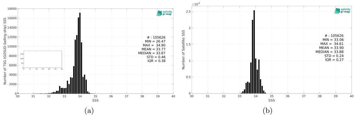
Figure 2: Histograms of SSS from TSG (GOSUD-Sailing-ship) (a) and SMOS SSS L4 v1 - Weekly (CMEMS-CNR) (b) considering all match-up pairs per bins of 0.1 over the Southern Ocean Pi-MEP region and for the full satellite product period.
