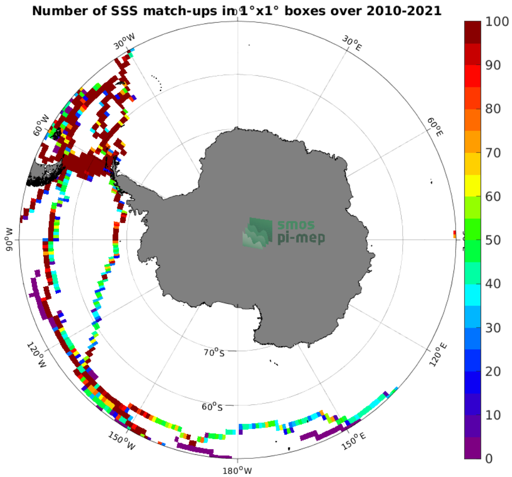
Figure 4: Number of SSS match-ups between TSG (GOSUD-Sailing-ship) SSS and the SMOS SSS L4 v1 - Weekly (CMEMS-CNR) SSS product for the Southern Ocean Pi-MEP region over 1^\circ \times 1^\circ boxes and for the full satellite product period.
