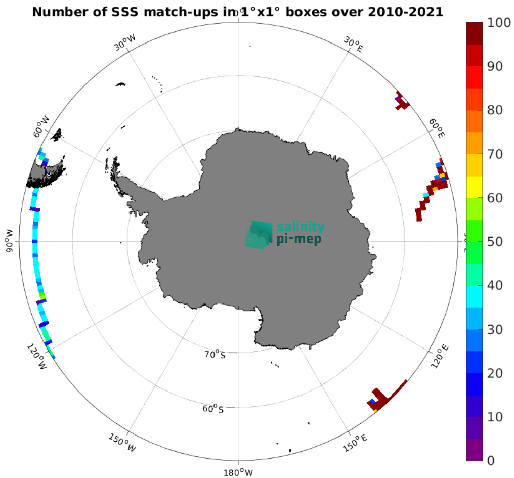
Figure 4: Number of SSS match-ups between TSG (GOSUD-Research-vessel) SSS and the SMOS SSS L4 v1 - Weekly (CMEMS-CNR) SSS product for the Southern Ocean Pi-MEP region over 1^\circ \times 1^\circ boxes and for the full satellite product period.
