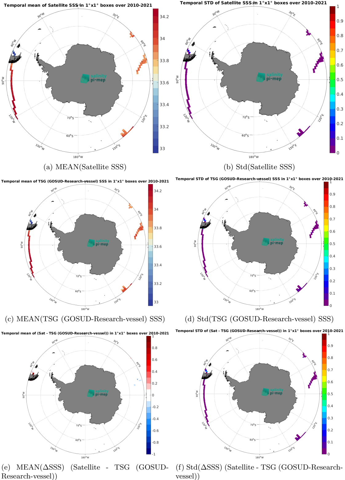
Figure 6: Temporal mean (left) and Std (right) of SSS from SMOS SSS L4 v1 - Weekly (CMEMS-CNR) (top), TSG (GOSUD-Research-vessel) (middle), and of \Delta SSS (Satellite - TSG (GOSUD-Research-vessel)). Only match-up pairs are used to generate these maps.
