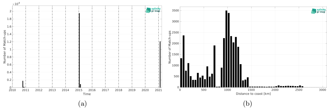
Figure 1: Number of match-ups between TSG (GOSUD-Research-vessel) and SMOS SSS L4 v1 - Weekly (CMEMS-CNR) SSS as a function of time (a) and as function of the distance to coast (b) over the Southern Ocean Pi-MEP region and for the full satellite product period.
