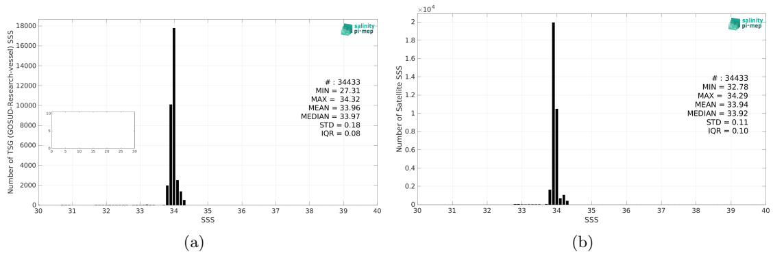
Figure 2: Histograms of SSS from TSG (GOSUD-Research-vessel) (a) and SMOS SSS L4 v1 - Weekly (CMEMS-CNR) (b) considering all match-up pairs per bins of 0.1 over the Southern Ocean Pi-MEP region and for the full satellite product period.
