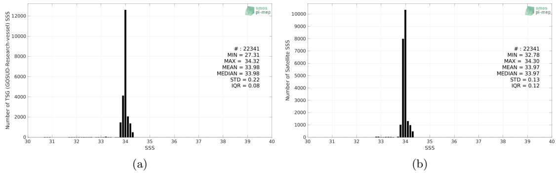
Figure 2: Histograms of SSS from TSG (GOSUD-Research-vessel) (a) and SMOS SSS L4 v1 - Weekly (CMEMS-CNR) (b) considering all match-up pairs per bins of 0.1 over the Southern Ocean Pi-MEP region and for the full satellite product period.
