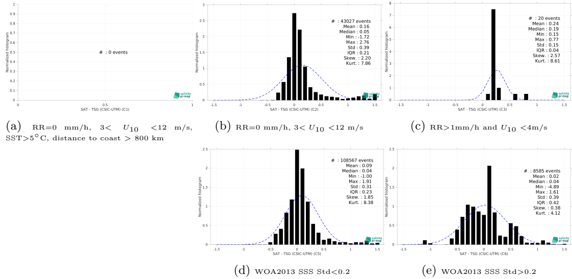
Figure 13: Normalized histogram of \Delta\text{SSS} (SMOS SSS L4 v1 - Weekly (CMEMS-CNR) - TSG (CSIC-UTM)) for 5 different subdatasets corresponding to: RR=0 mm/h, 3 < U_{10} < 12 m/s, SST >5^{\circ}\text{C} , distance to coast > 800 km (a), RR=0 mm/h, 3 < U_{10} < 12 m/s (b), RR>1\text{mm/h} and U_{10} < 4\text{m/s} (c), WOA2013 SSS Std <0.2 (d), WOA2013 SSS Std >0.2 (e).
