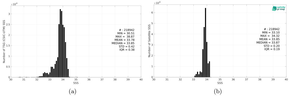
Figure 2: Histograms of SSS from TSG (CSIC-UTM) (a) and SMOS SSS L4 v1 - Weekly (CMEMS-CNR) (b) considering all match-up pairs per bins of 0.1 over the Southern Ocean Pi-MEP region and for the full satellite product period.
