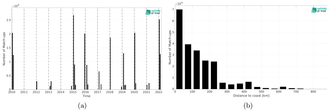
Figure 1: Number of match-ups between TSG (CSIC-UTM) and SMOS SSS L4 v1 - Weekly (CMEMS-CNR) SSS as a function of time (a) and as function of the distance to coast (b) over the Southern Ocean Pi-MEP region and for the full satellite product period.
