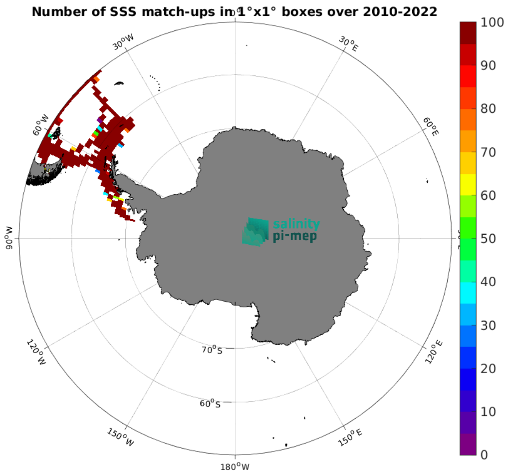
Figure 4: Number of SSS match-ups between TSG (CSIC-UTM) SSS and the SMOS SSS L4 v1 - Weekly (CMEMS-CNR) SSS product for the Southern Ocean Pi-MEP region over 1^{\circ} \times 1^{\circ} boxes and for the full satellite product period.
