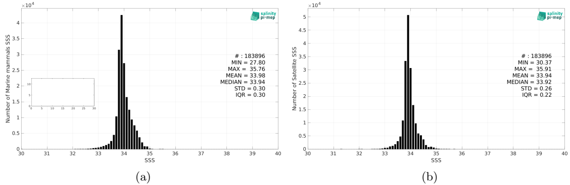
Figure 2: Histograms of SSS from Marine mammals (a) and SMOS SSS L4 v1 - Weekly (CMEMS-CNR) (b) considering all match-up pairs per bins of 0.1 over the Southern Ocean Pi-MEP region and for the full satellite product period.
