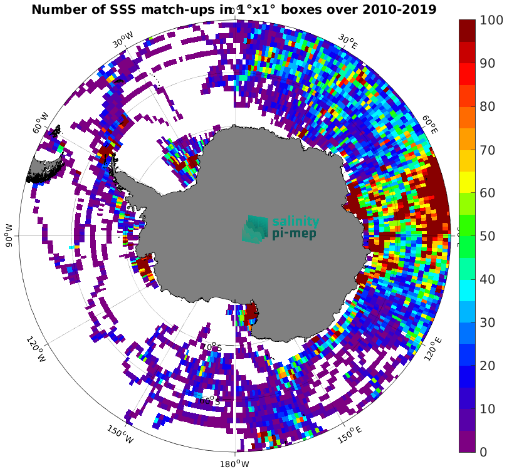
Figure 4: Number of SSS match-ups between Marine mammals SSS and the SMOS SSS L4 v1 - Weekly (CMEMS-CNR) SSS product for the Southern Ocean Pi-MEP region over 1^\circ \times 1^\circ boxes and for the full satellite product period.
