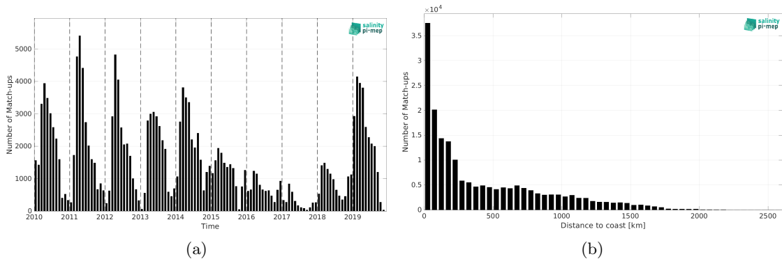
Figure 1: Number of match-ups between Marine mammals and SMOS SSS L4 v1 - Weekly (CMEMS-CNR) SSS as a function of time (a) and as function of the distance to coast (b) over the Southern Ocean Pi-MEP region and for the full satellite product period.
