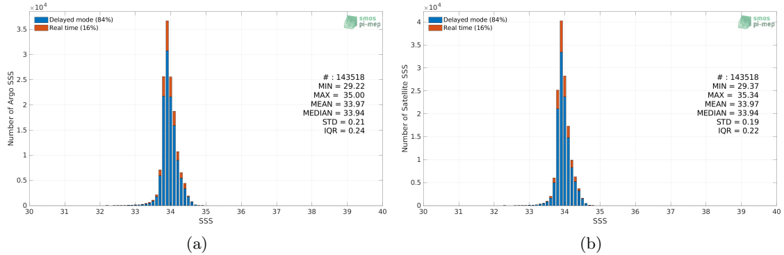
Figure 2: Histograms of SSS from Argo (a) and SMOS SSS L4 v1 - Weekly (CMEMS-CNR) (b) considering all match-up pairs per bins of 0.1 over the Southern Ocean Pi-MEP region and for the full satellite product period.
