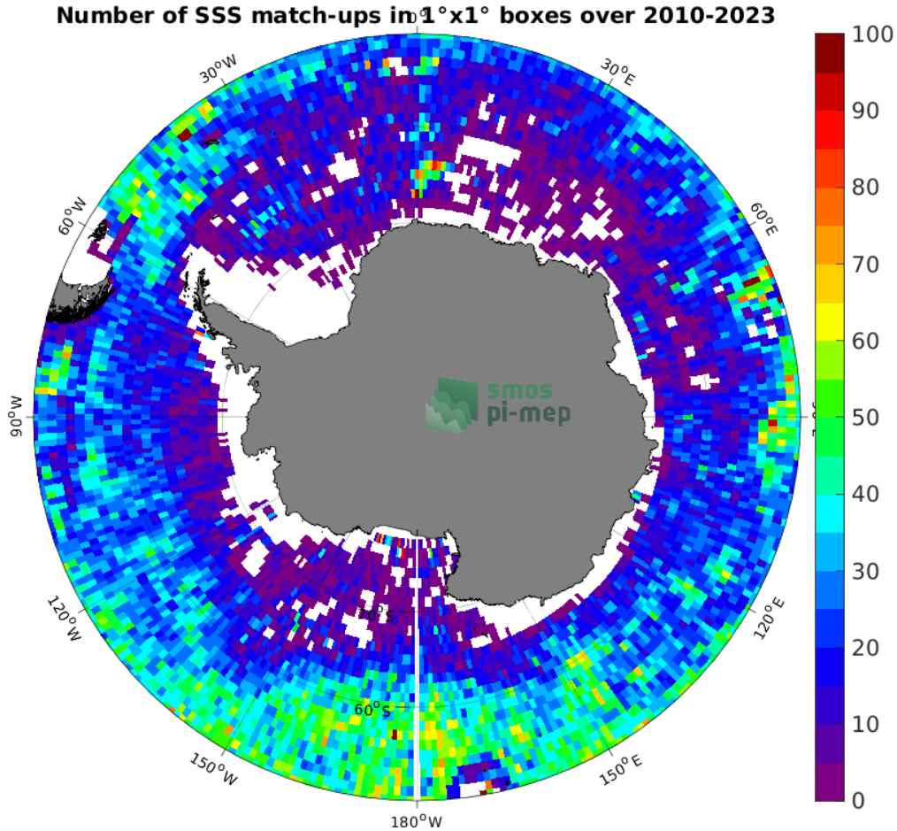
Figure 4: Number of SSS match-ups between Argo SSS and the SMOS SSS L4 v1 - Weekly (CMEMS-CNR) SSS product for the Southern Ocean Pi-MEP region over 1^\circ \times 1^\circ boxes and for the full satellite product period.
