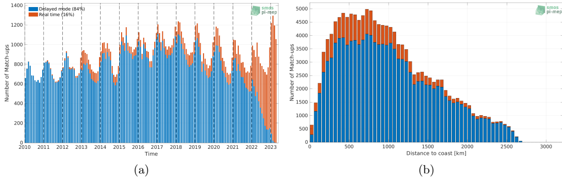
Figure 1: Number of match-ups between Argo and SMOS SSS L4 v1 - Weekly (CMEMS-CNR) SSS as a function of time (a) and as function of the distance to coast (b) over the Southern Ocean Pi-MEP region and for the full satellite product period.
