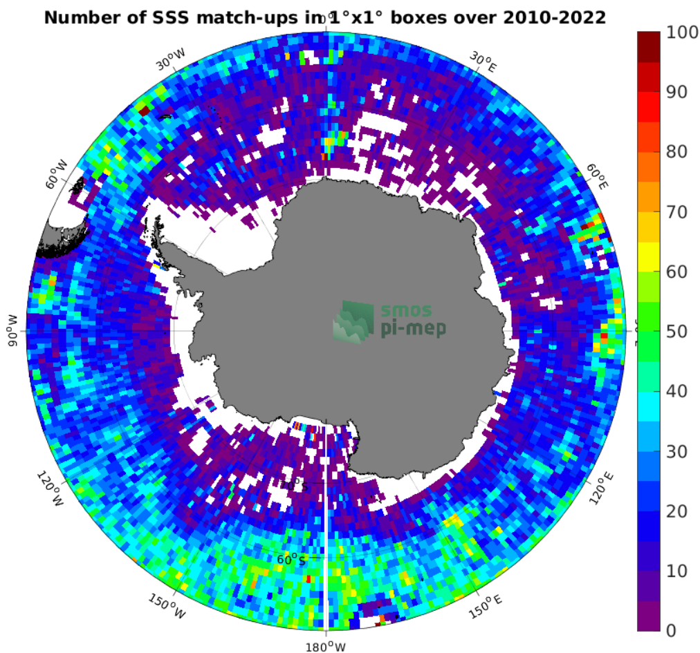
Figure 4: Number of SSS match-ups between Argo SSS and the SMOS SSS L4 v1 - Weekly (CMEMS-CNR) SSS product for the Southern Ocean Pi-MEP region over 1^\circ \times 1^\circ boxes and for the full satellite product period.
