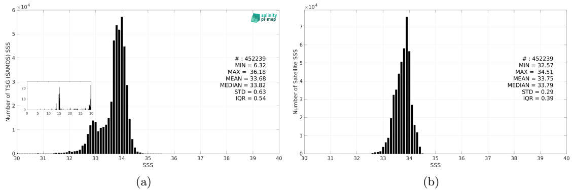
Figure 3: Histograms of SSS from TSG (SAMOS) (a) and SMOS SSS L4 v1 - Monthly (CMEMS-CNR) (b) considering all match-up pairs per bins of 0.1 over the Southern Ocean Pi-MEP region and for the full satellite product period.
