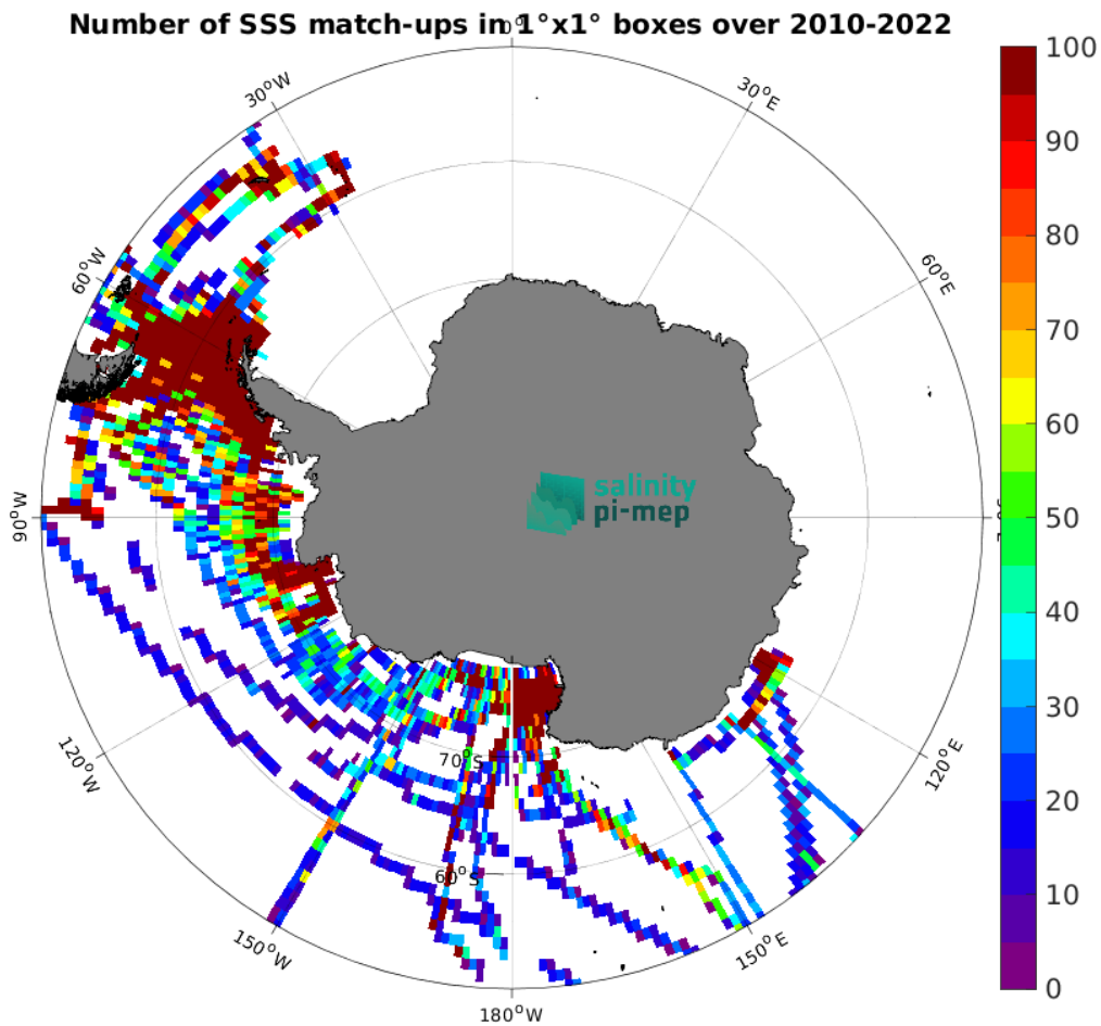
Figure 5: Number of SSS match-ups between TSG (SAMOS) SSS and the SMOS SSS L4 v1 - Monthly (CMEMS-CNR) SSS product for the Southern Ocean Pi-MEP region over 1^\circ \times 1^\circ boxes and for the full satellite product period.
