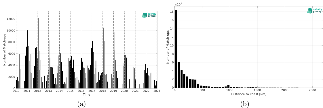
Figure 2: Number of match-ups between TSG (SAMOS) and SMOS SSS L4 v1 - Monthly (CMEMS-CNR) SSS as a function of time (a) and as function of the distance to coast (b) over the Southern Ocean Pi-MEP region and for the full satellite product period.
